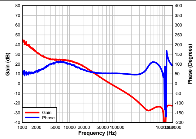
图 7-7. Bode Plot V IN = 12 V I OUT = 3 A
