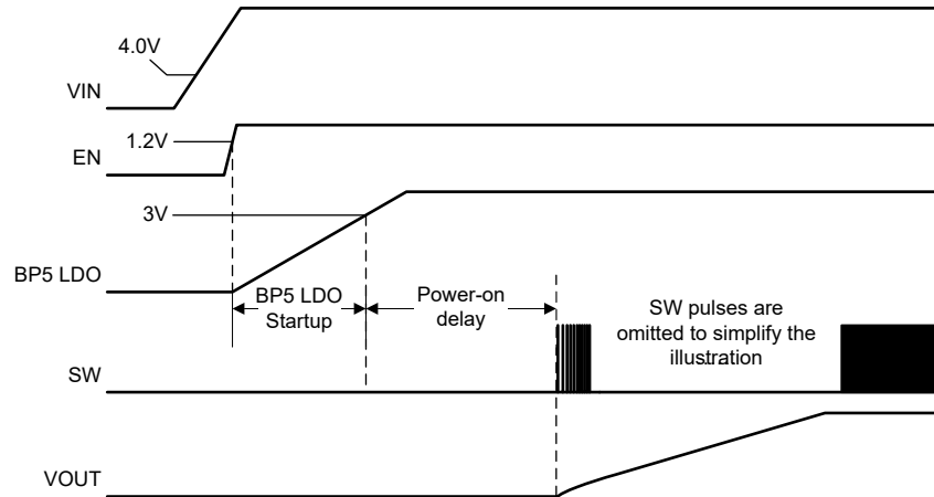
图 6-1. Start-Up Sequence
