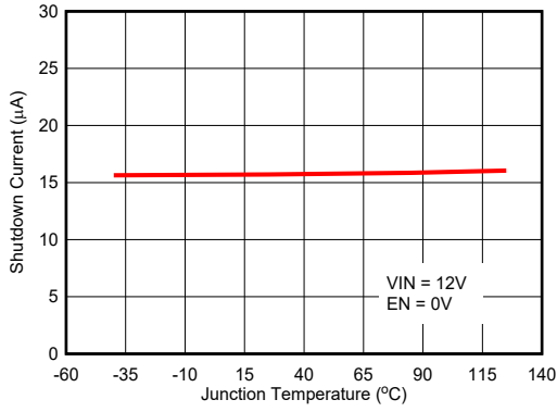
图 5-13. Shutdown Current
