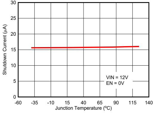
图 5-13. Shutdown Current
