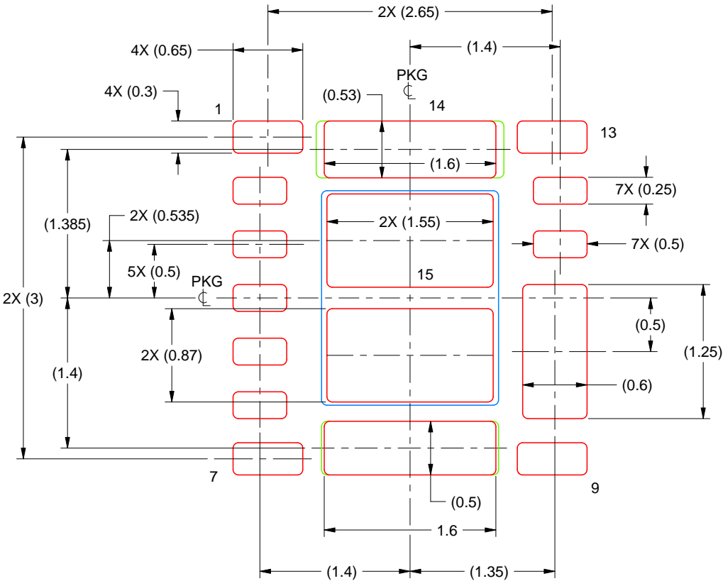
SOLDER PASTE EXAMPLE BASED ON 0.125 mm THICK STENCIL SCALE:20X PRINTED SOLDER COVERAGE BY AREA UNDER PACKAGE PAD 8: 97% PAD 14: 91% PAD 15: 82%
