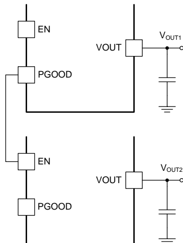
图 22. Sequencing Schematic
