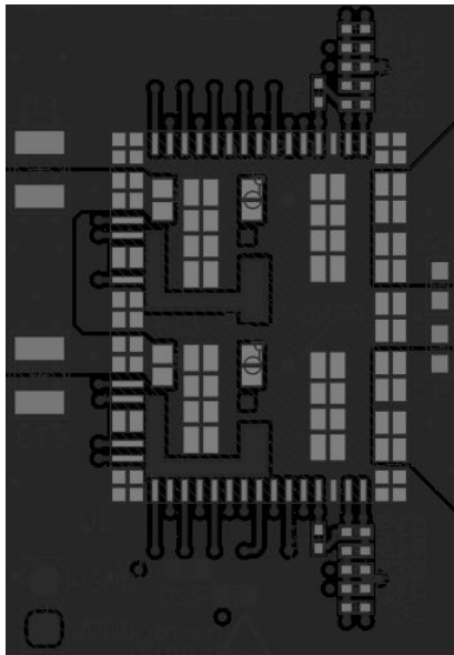
图 7-21. Top-Layer Layout (Top View)
