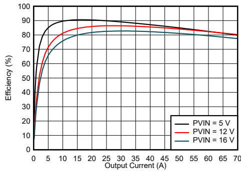
图 7-10. Efficiency vs Output Current
