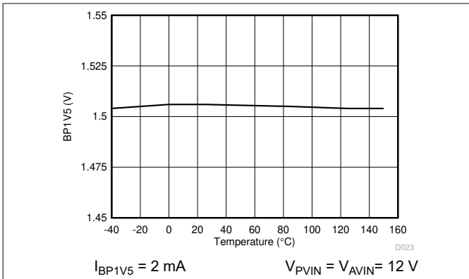
图 5-13. BP1V5 Voltage vs Junction Temperature
