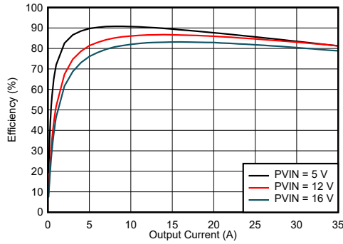
图 7-1. Efficiency vs Output Current
