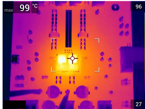
图 7-24. Thermal Image at 25^\circ\text{C} Ambient, 12 Vin, 0.8 Vout, 70 A, 550 kHz
