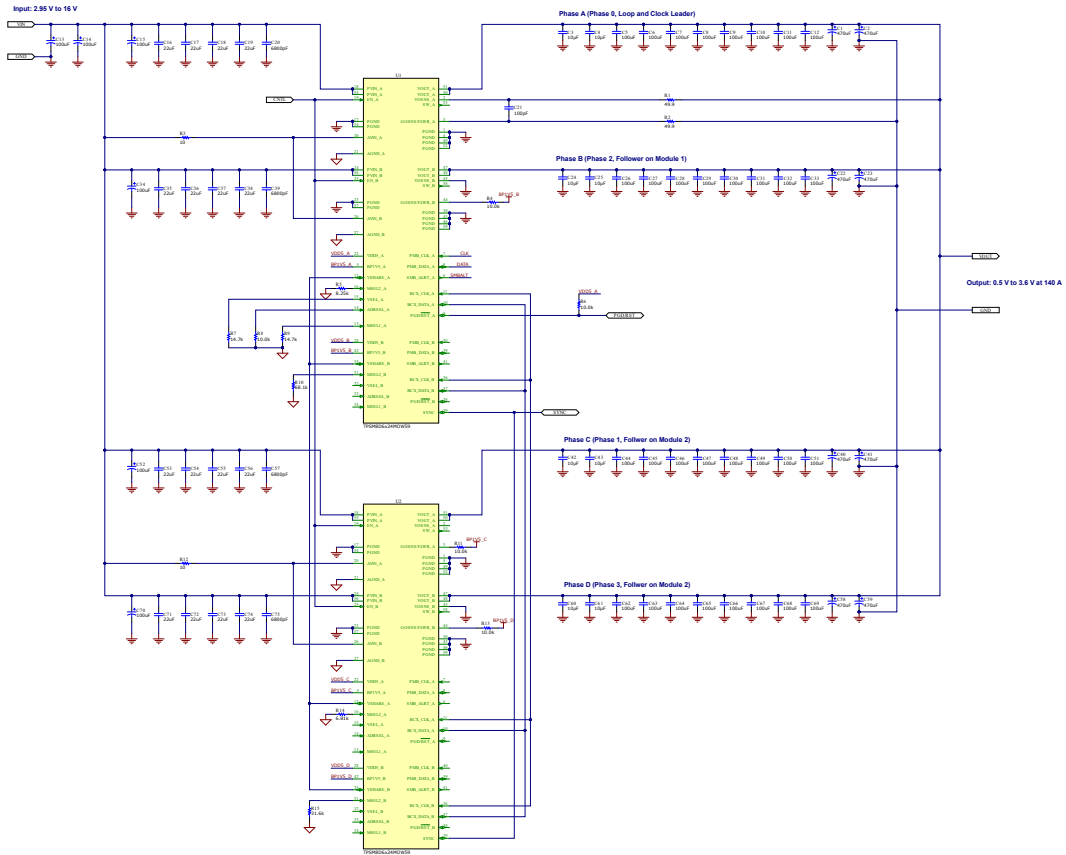
图 7-18. TPSM8D6C24 Four-Phase Application
