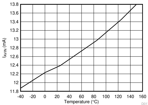
图 5-11. Nonswitching Input Current ( I_{AVIN} ) vs Junction Temperature
