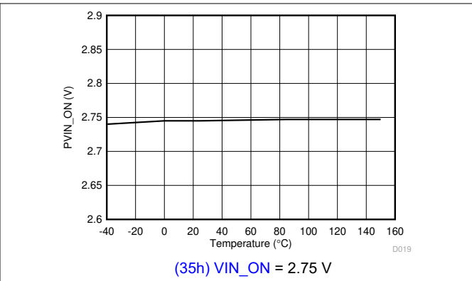
图 5-14. Turn-On Voltage vs Junction Temperature
