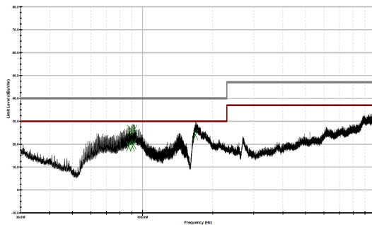
图 7-25. Radiated Emissions 12-V Input, 1.0-V Outputs, 35-A/Output Load
