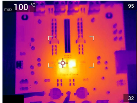
图 7-23. Thermal Image at 25^\circ\text{C} Ambient, 12 Vin, 0.8V and 1.2 Vout, 35 A, 550 kHz
