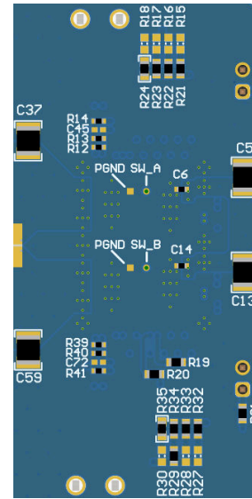
图 7-20. Bottom-Layer Components (Top View)
