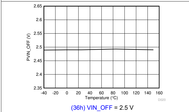
图 5-15. Turn-Off Voltage vs Junction Temperature
