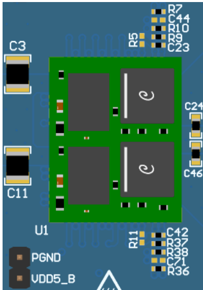
图 7-19. Top-Layer Components (Top View)
