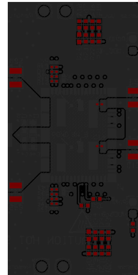
图 7-22. Bottom-Layer Layout (Top View)
