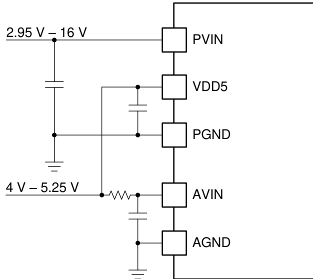
图 6-3. TPSM8D6C24 Separate PVIN and AVIN Connections with VDD5
