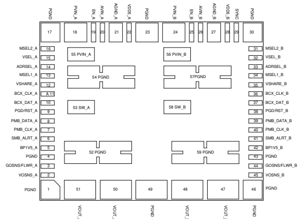
图 4-2. 59-Pin QFM-MOW Package (Bottom View)
