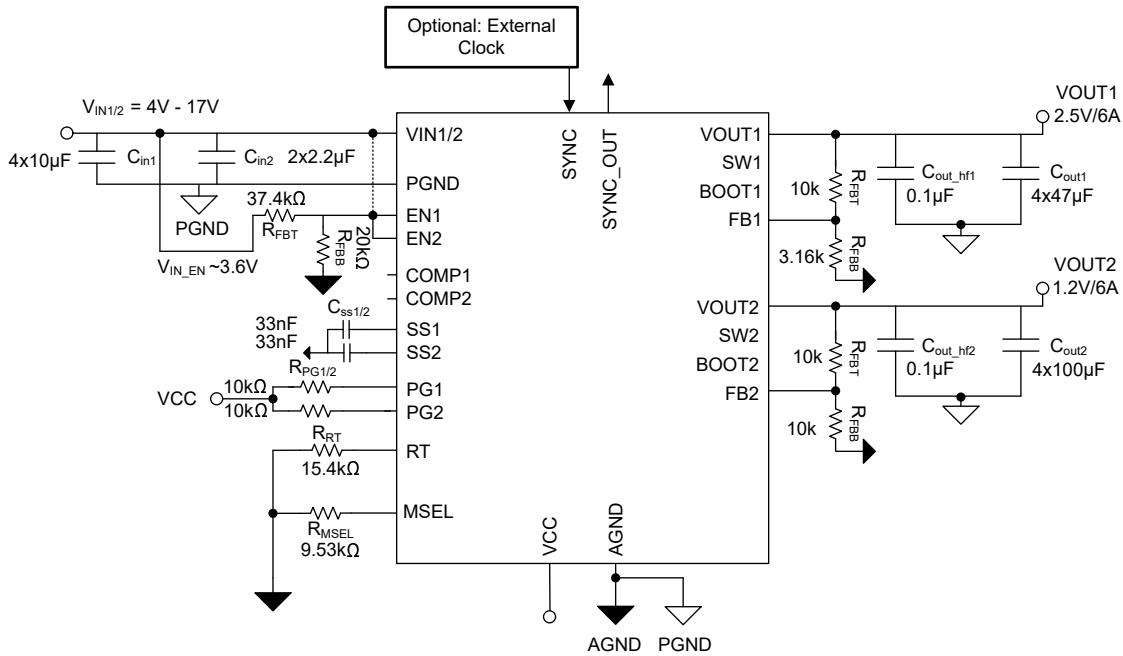
Figure 8-1. Two Output Application Schematic
