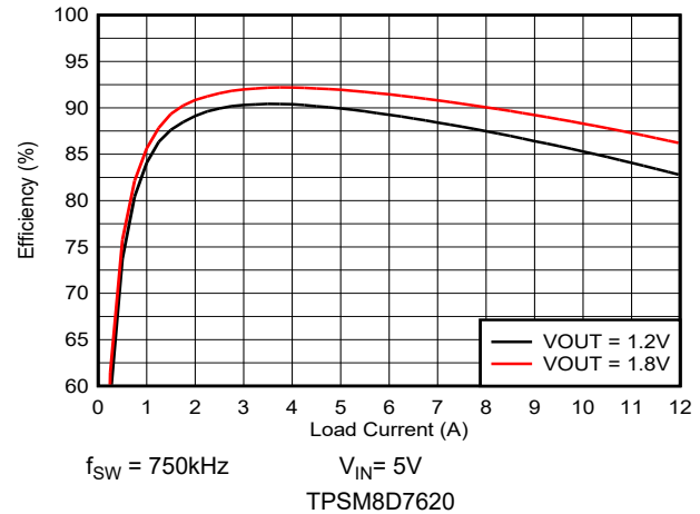
Figure 8-22. Efficiency vs Output Current
