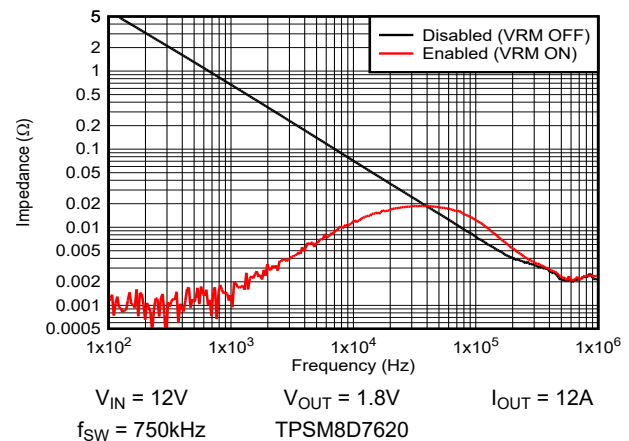
Figure 8-24. VOUT1 Output Impedance
