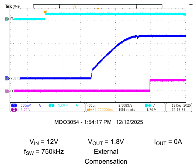
Figure 8-26. Startup From EN
