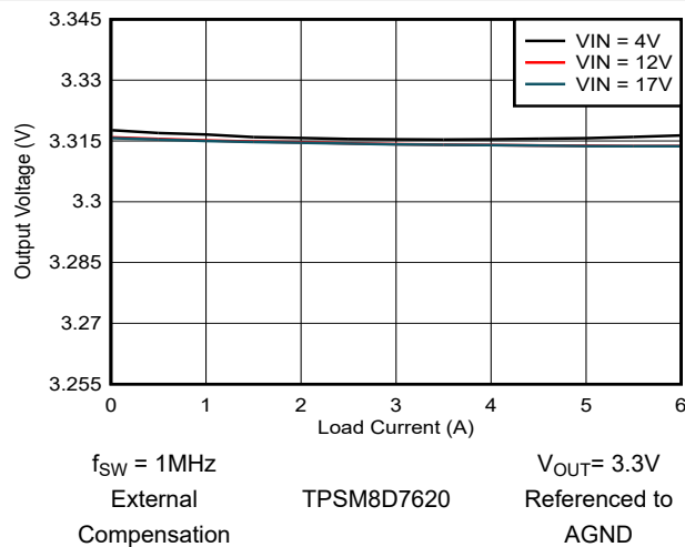
Figure 8-6. Load Regulation
