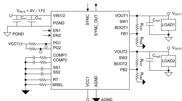
Typical Schematic
