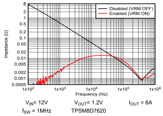
Figure 8-11. VOUT2 Output Impedance
