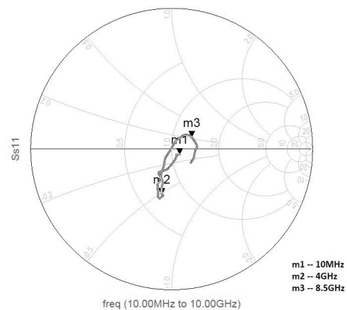
图 6-30. Single-Ended S11
