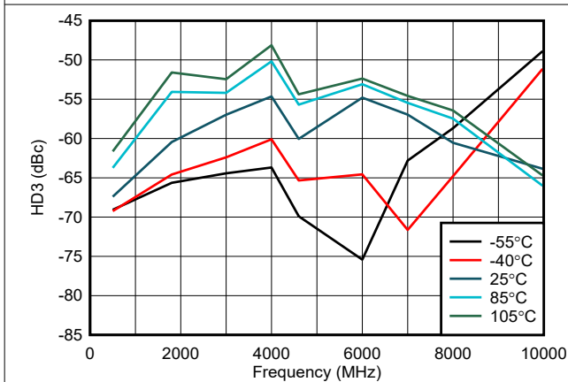
P_O = +3\text{dBm}
