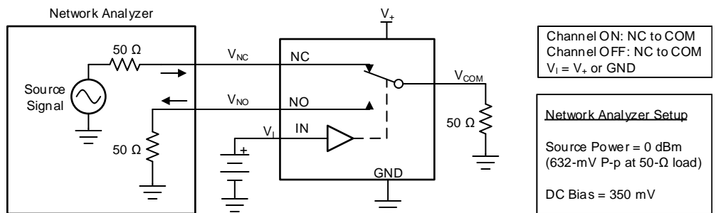
Figure 22. Crosstalk ( X_{TALK} )
