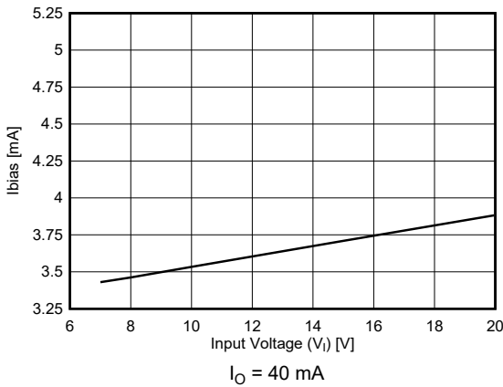
图 6-15. Bias Current vs Input Voltage for New Chip at T_J = 25\text{ }^\circ\text{C}
