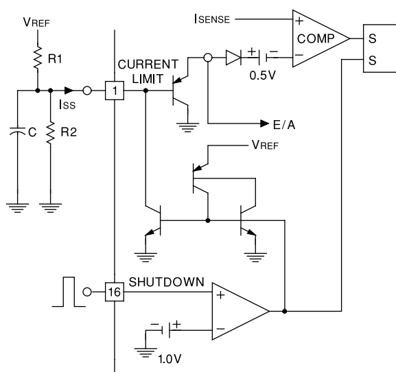
Figure 6. Shutdown Latch
