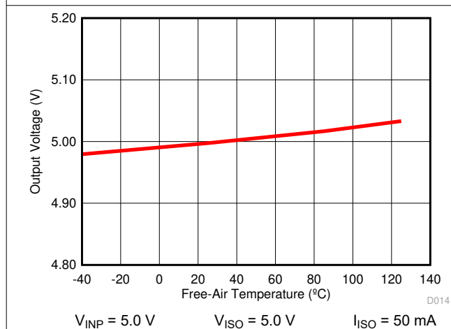
图 6-20. Isolated Supply Voltage ( V_{ISO} ) vs Free-Air Temperature
