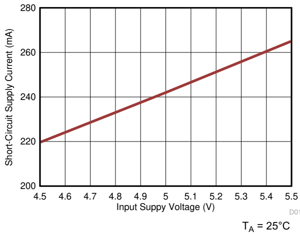
图 6-24. Short-Circuit Supply Current ( I_{VIN\_SC} ) vs Supply Voltage ( V_{INP} )
