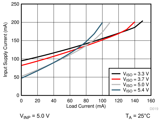
图 6-25. Input Supply Current ( I_{VINP} ) vs Load Current ( I_{ISO} )
