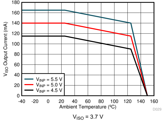
图 6-11. Maximum V ISO Output Current vs. Temperature
