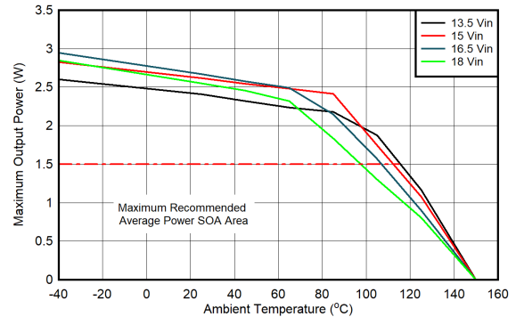
图 6-3. SOA 降额曲线: V_{\text{DDD-VEE}} = 18\text{V} , V_{\text{COM-VEE}} = 3\text{V} , T_{\text{shut}} = 160^{\circ}\text{C} , V_{\text{COM-VEE}} 无负载
