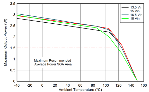
图 6-5. SOA 降额曲线: V_{\text{DDD-VEE}} = 25\text{V} , V_{\text{COM-VEE}} = 5\text{V} , T_{\text{shut}} = 160^{\circ}\text{C} , V_{\text{COM-VEE}} 无负载
