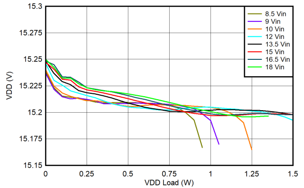
图 6-29. UCC14341B-Q1 V_{VDD-VEE} 负载调节 : T_{AMBIENT} = 85^{\circ}C , V_{VDD-VEE} = 15V , V_{COM-VEE} = 4V
