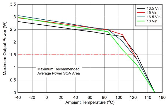
图 6-4. SOA 降额曲线: V_{\text{DDD-VEE}} = 22\text{V} , V_{\text{COM-VEE}} = 4\text{V} , T_{\text{shut}} = 160^{\circ}\text{C} , V_{\text{COM-VEE}} 无负载
