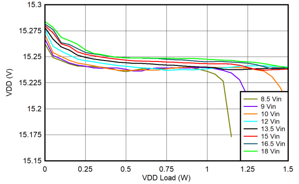
图 6-27. UCC14341B-Q1 V_{VDD-VEE} 负载调节 : T_{AMBIENT} = -40^{\circ}C , V_{VDD-VEE} = 15V , V_{COM-VEE} = 4V
