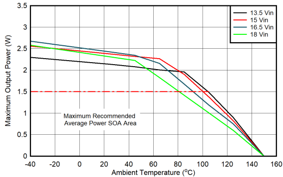
图 6-2. SOA 降额曲线: V_{\text{DDD-VEE}} = 15\text{V} , V_{\text{COM-VEE}} = 5\text{V} , T_{\text{shut}} = 160^{\circ}\text{C} , V_{\text{COM-VEE}} 无负载
