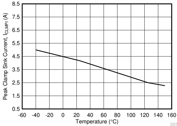
图 5-22. I_{CLMPI} Miller Clamp Sink Current vs. Temperature
