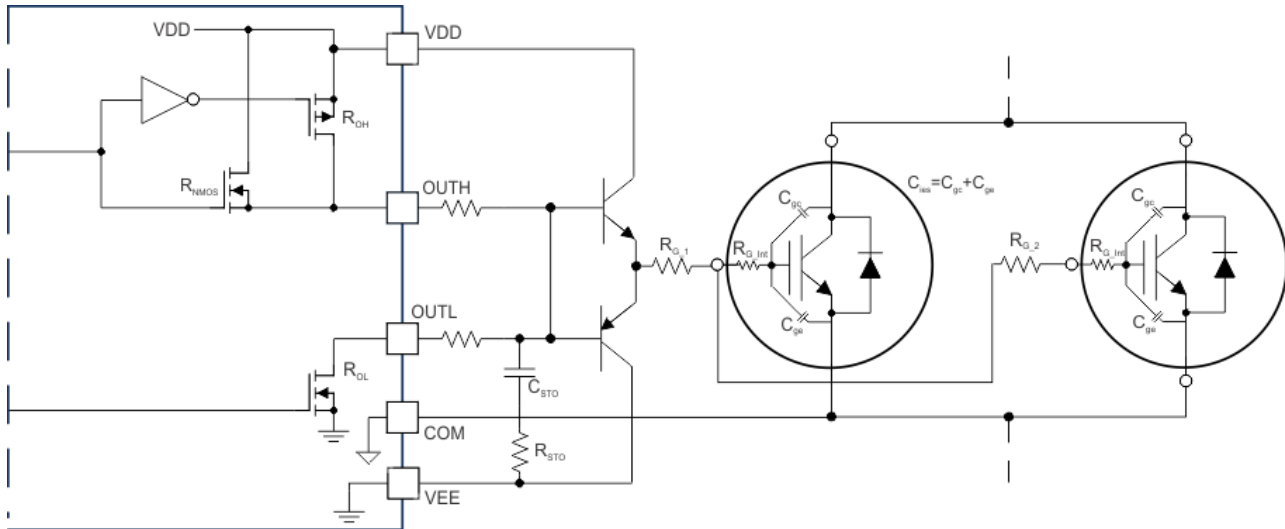
图 8-16. Current Buffer for Increased Drive Strength
