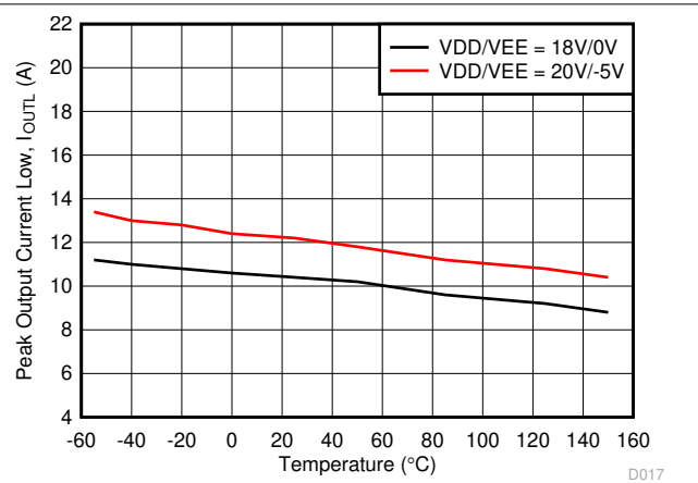
图 5-5. Output Low Driver Current vs. Temperature
