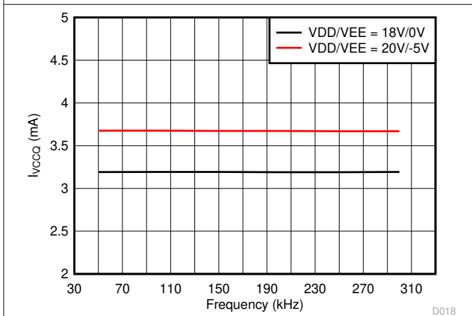
图 5-8. I VCCQ Supply Current vs. Input Frequency
