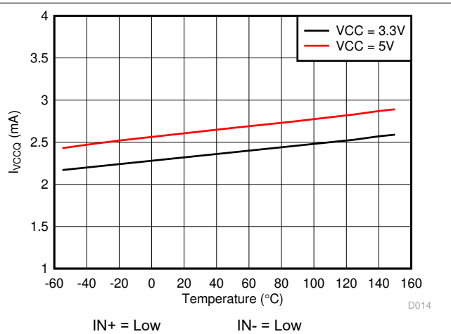
图 5-7. I VCCQ Supply Current vs. Temperature
