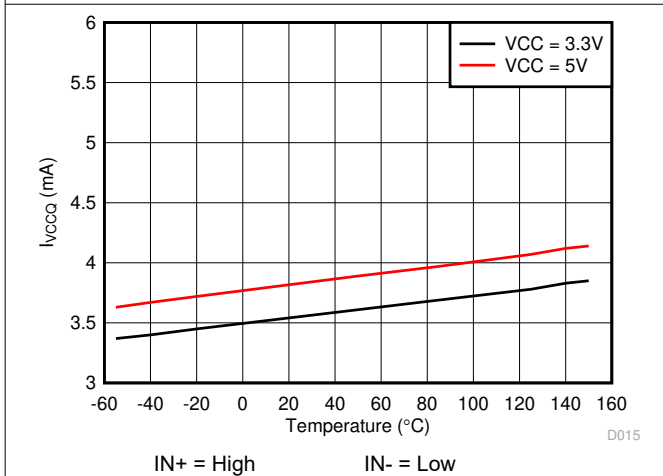
图 5-6. I VCCQ Supply Current vs. Temperature
