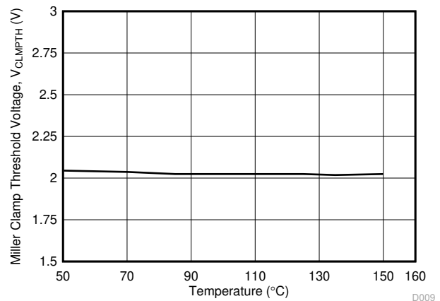
图 5-21. V_{CLMPH} Miller Clamp Threshold Voltage vs. Temperature
