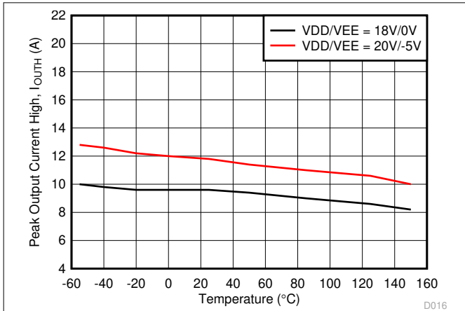
图 5-4. Output High Drive Current vs. Temperature
