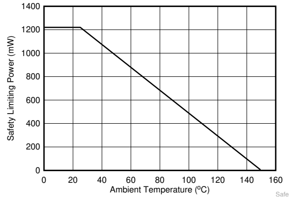
图 5-2. Thermal Derating Curve for Limiting Power per VDE
