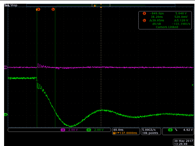
A. V_{DD} = V_{HB} = 6\text{ V} , HS = C_{LOAD} = 10\text{ nF} Ch4 = LO VSS
