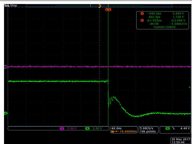
V_{DD} = V_{HB} = 6\text{ V} , HS = C_{LOAD} = 10\text{ nF} Ch4 = HO VSS
