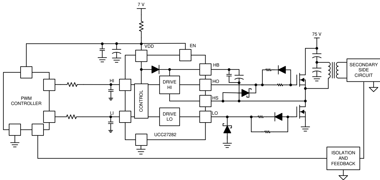
图 8-1. Typical Application
