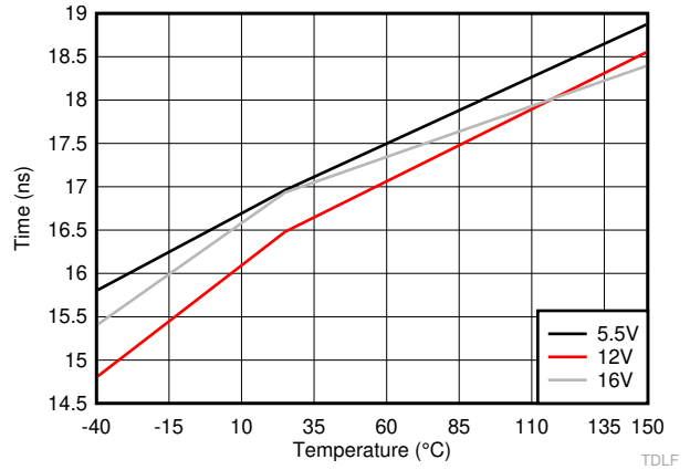
图 6-26. LO Falling Propagation Delay (TDLFF)
