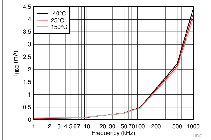
图 6-4. HB Operating Current
