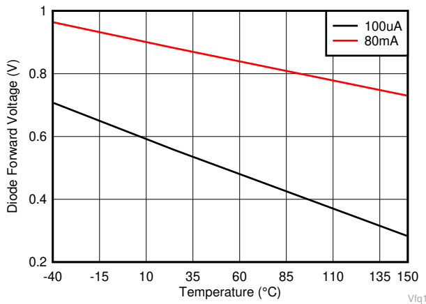
图 6-11. Boot Diode Forward Voltage Drop
