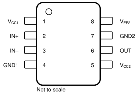
图 5-3. UCC5320E and UCC5390E 8-Pin SOIC Top View
