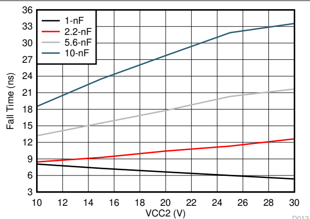
图 6-41. UCC5350SBD Fall Time vs C_L and V_{CC2}
