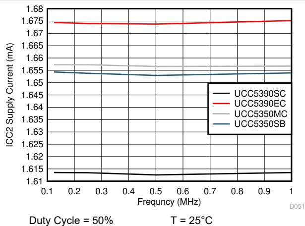
图 6-21. I_{CC2} Supply Current vs Input Frequency
