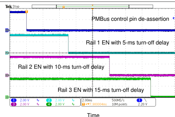
Figure 7-4. Shut-Down Waveforms
