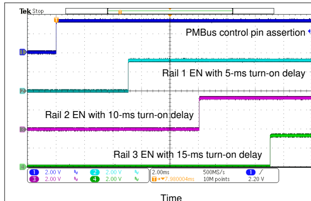
Figure 7-3. Start-Up Waveforms
