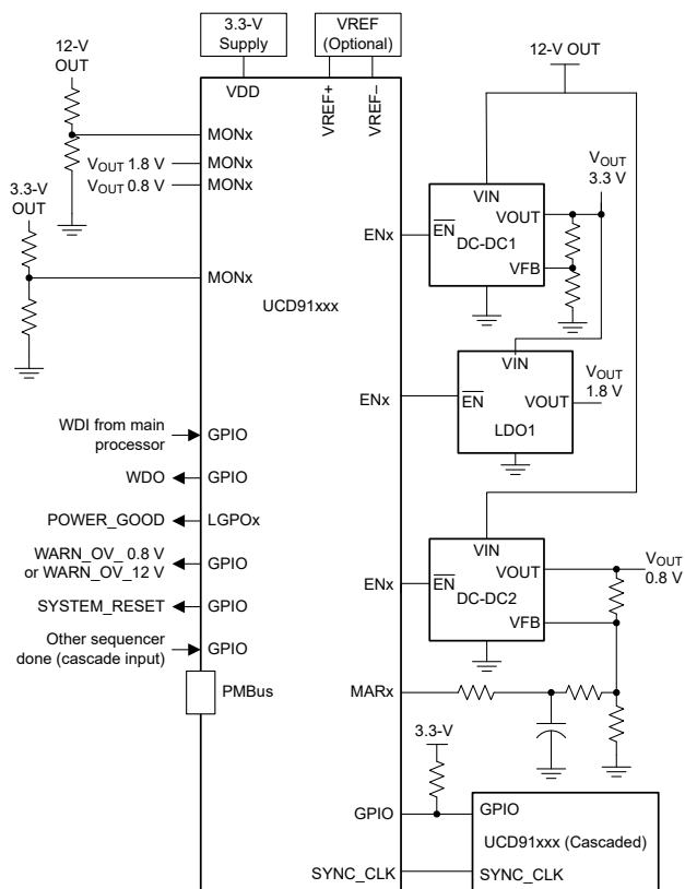
Figure 3-1. Simplified Application Diagram
