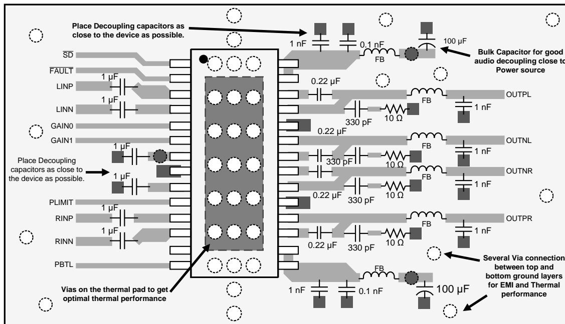
Figure 48. TPA3110D2 PCB Layout
