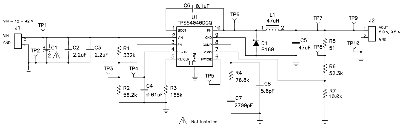
Figure 14. TPS54040EVM-456 Schematic
