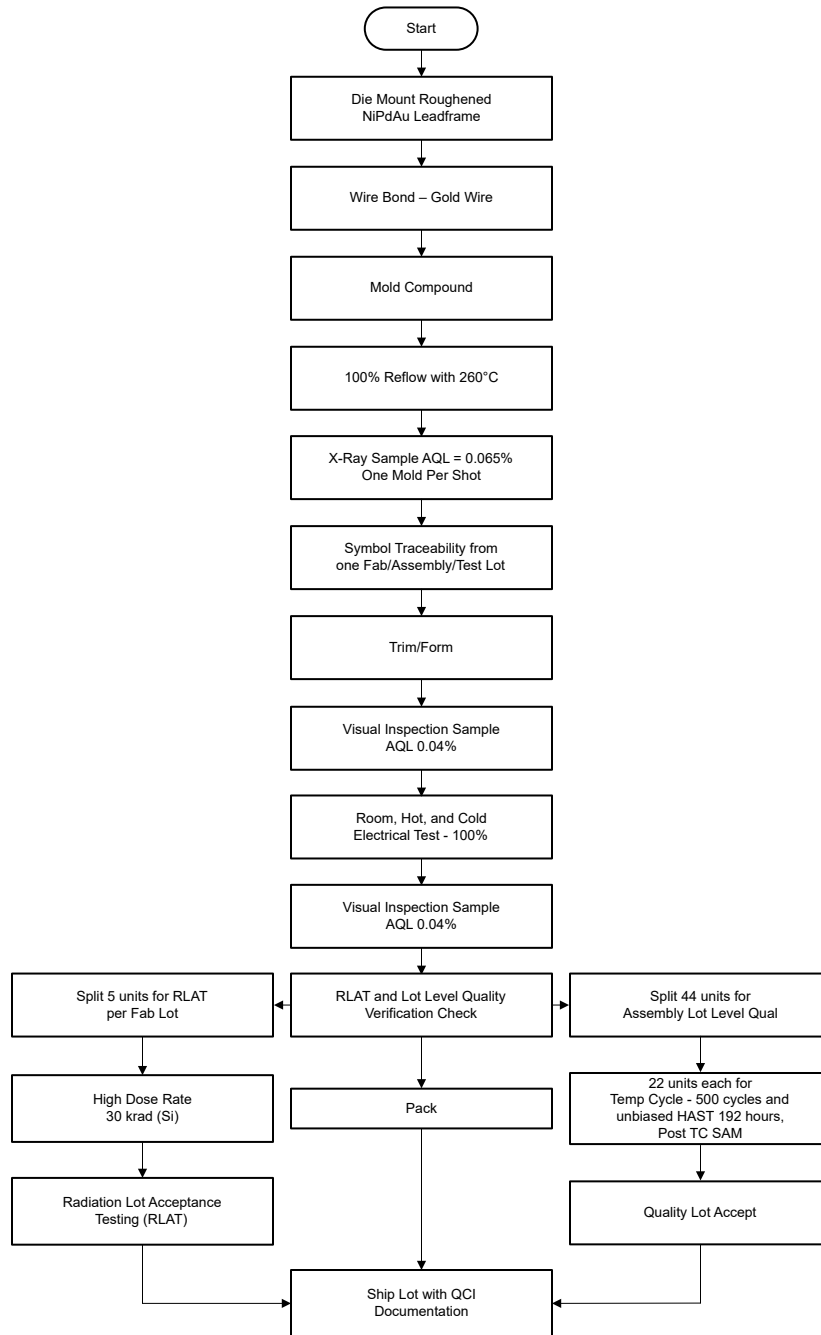
Figure 2-1. INA950-SEP Space Enhanced Plastic Production Flow Chart
