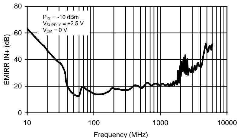
Figure 1. OPA357 EMIRR IN+ vs Frequency
