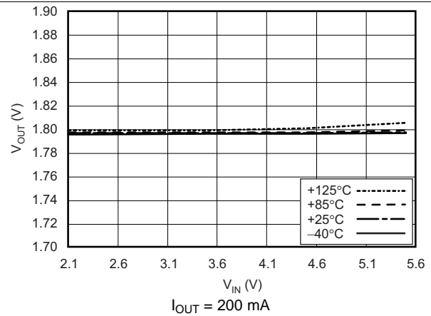
Figure 2. Line Regulation (TPS72718)
