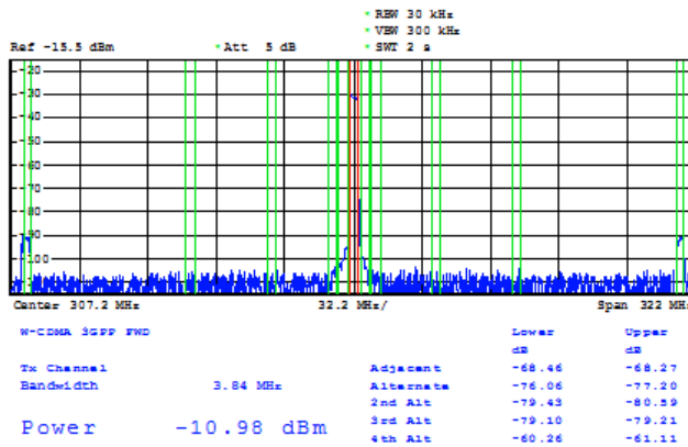
Figure 16. WCDMA; PLL enabled, F_{DAC} = 1228.8 MHz, IF = Fs/4 , N = 1 , PFD frequency = 153.6 MHz
