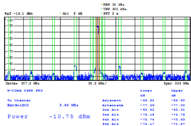
Figure 17. WCDMA 10 MHz; PLL enabled, F_{DAC} = 1228.8 MHz, IF = Fs/4 , N = 1 , PFD frequency = 38.4 MHz
