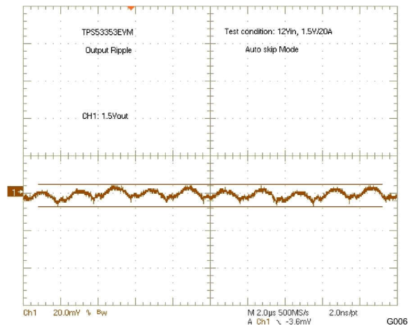
Figure 7-6. Output Ripple
