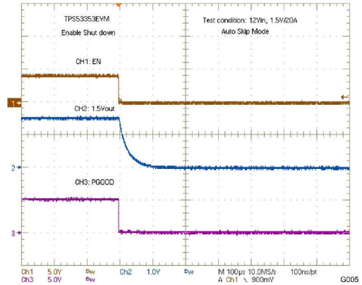
Figure 7-5. Enable Turn-Off
