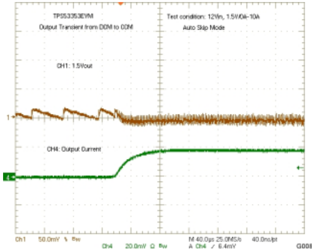
Figure 7-8. Output Transient From DCM to CCM
