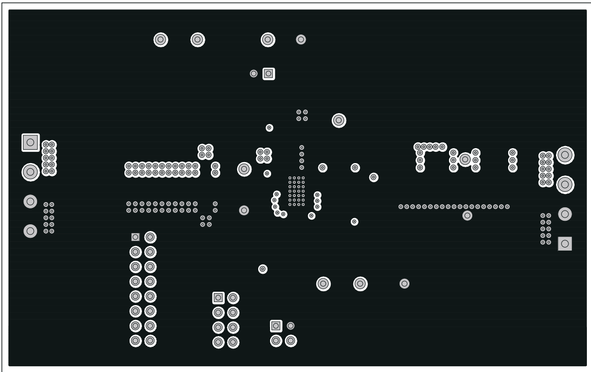
Figure 8-5. TPS53353EVM-744 Layer-3 Copper
