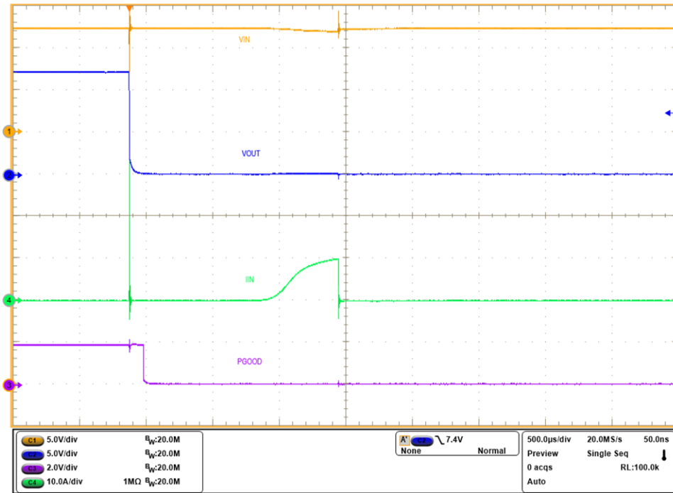
Figure 5. Output Hot-short response of TPS2598240 device
