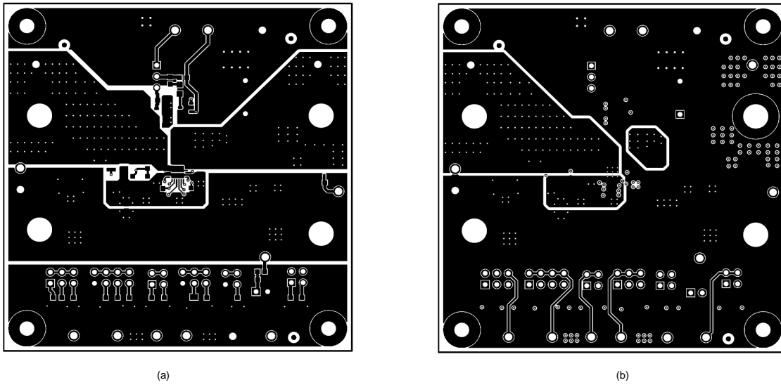
Figure 9. TPS259824OEVm Board (a) Top Layer (b) Bottom Layer
