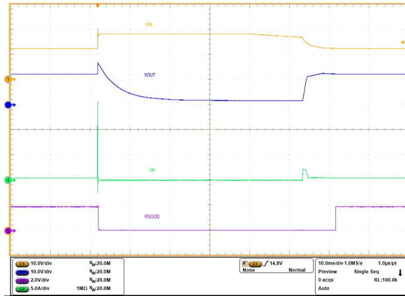
Figure 7. Over Voltage Protection Response of TPS2598240 Device
