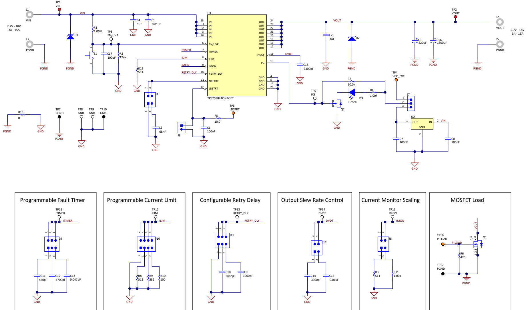
Figure 1. TPS259824OEVM eFuse Evaluation Board Schematic
