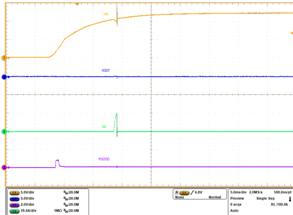
Figure 6. Test Waveform of Wakeup Into Output Short for TPS2598240 Device
