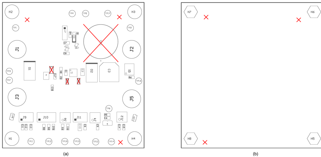
Figure 8. TPS2598240EVM Board (a) Top Assembly (b) Bottom Assembly
