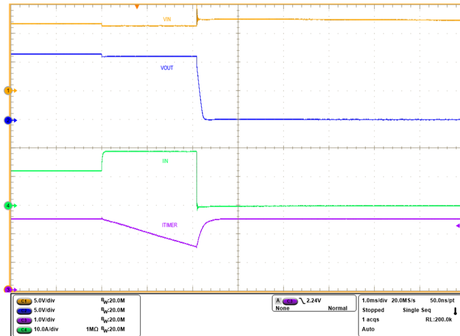
Figure 4. Over Current Response of TPS2598240 for 15 A Current Limit Setting
