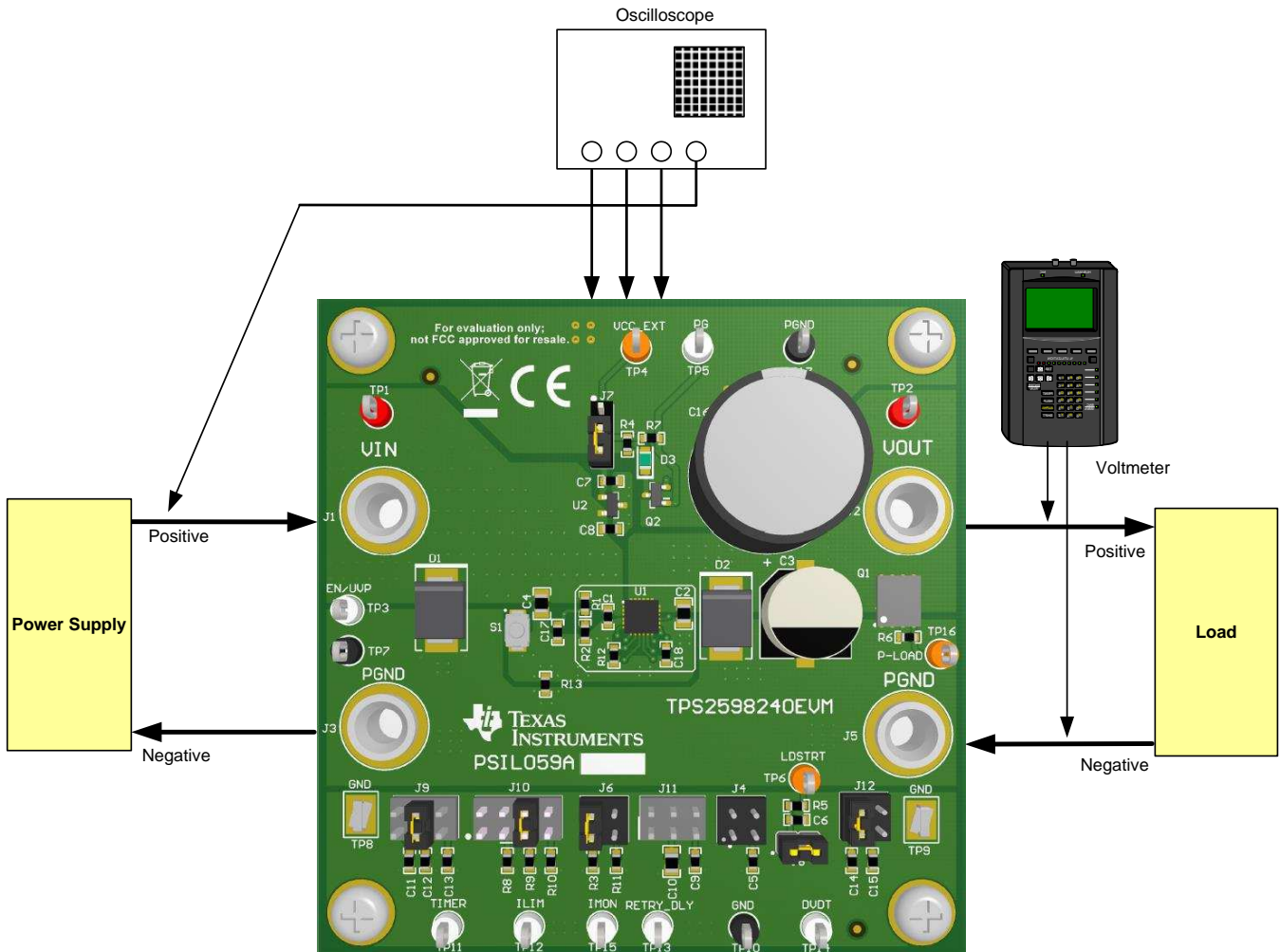
Figure 2. TPS259824OEVm Setup with Test Equipment
