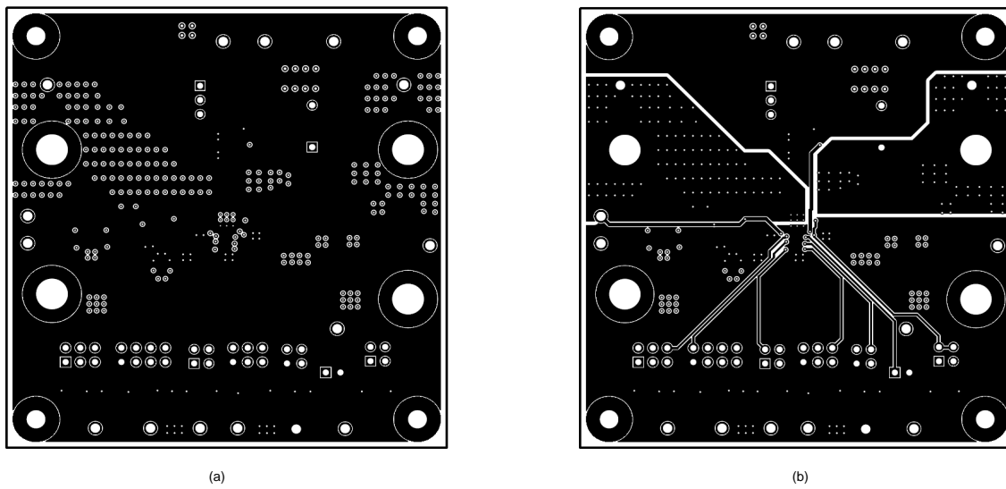
Figure 10. TPS259824OEVm Board (a) Inner Signal Layer (b) Inner Routing Layer
