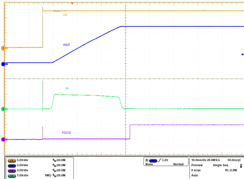
Figure 3. TPS259824O Output Rise Profile (VIN = 12 V, CdVdT = 10 nF, COUT = 2 mF, No-load)
