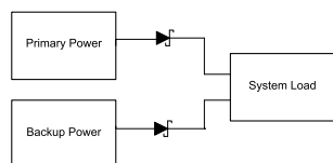
Figure 1. Diode ORing Configuration
