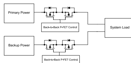
Figure 2. Discrete P-Channel MOSFET Power MUXing Configuration
