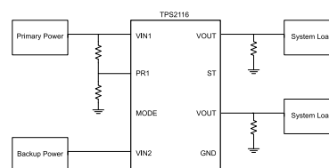
Figure 3. TPS2116 Power MUX
