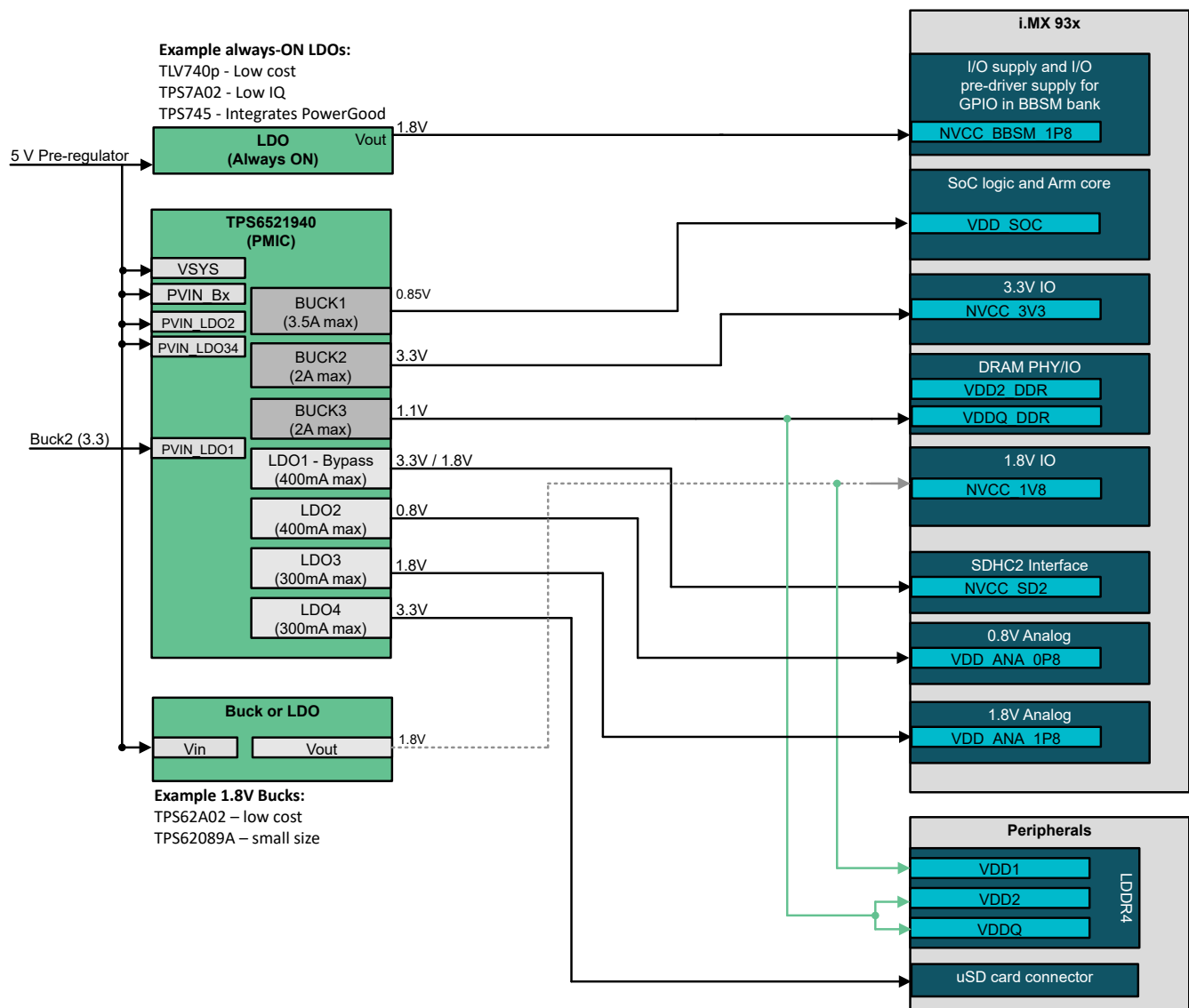
Figure 2-1. TPS6521940 Example Power Block Diagram
