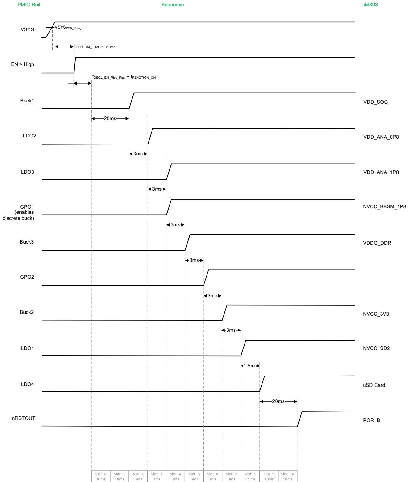
Figure 2-2. TPS6521940 Power-Up Sequence
