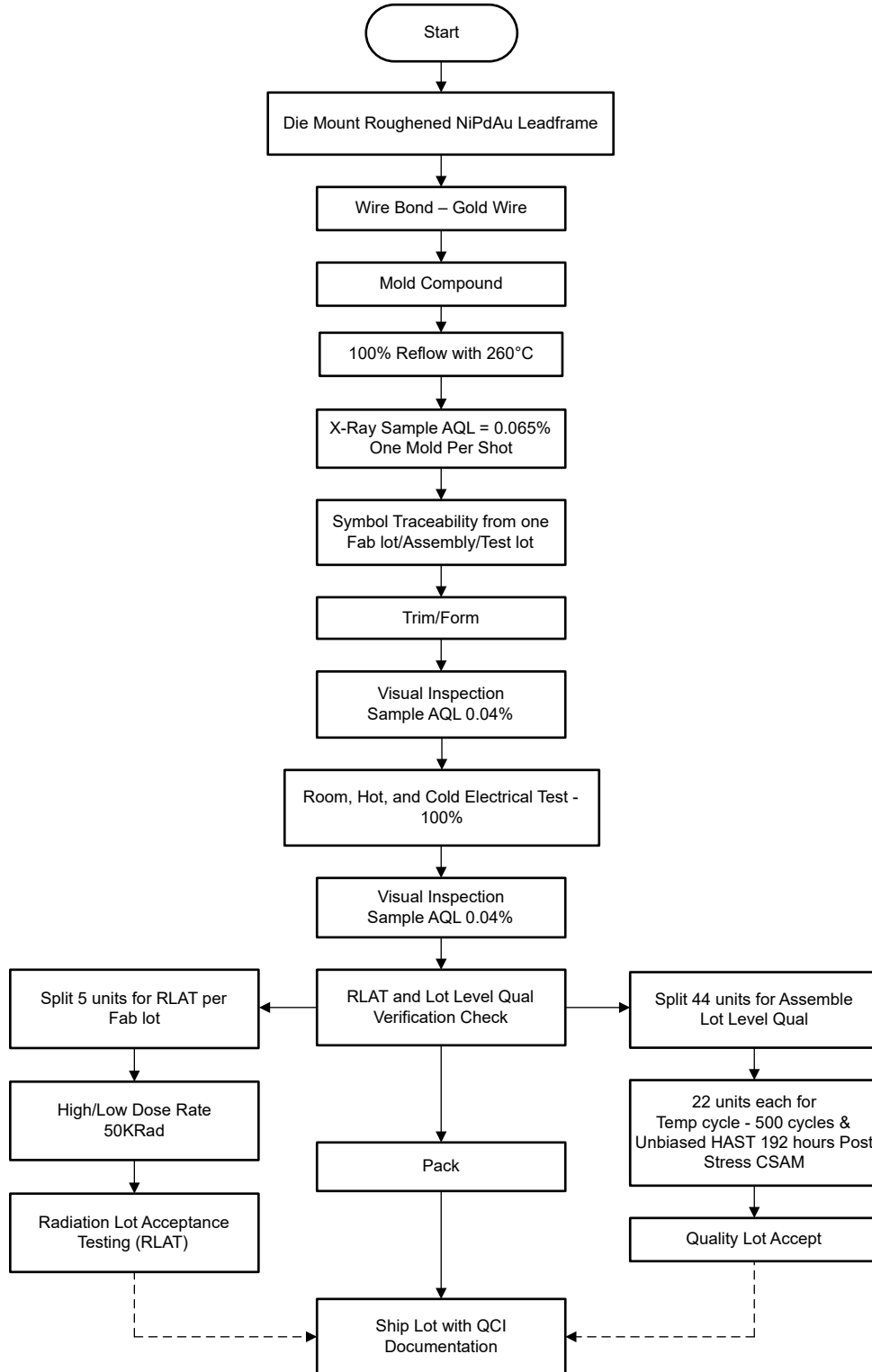
Figure 2-1. TPS7H60x5-SEP Space Enhanced Plastic Production Flow Chart
