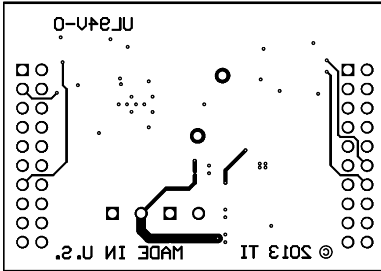
Figure 11. Bottom Layer Routing
