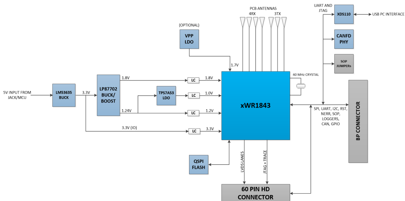
Figure 3. Block Diagram
