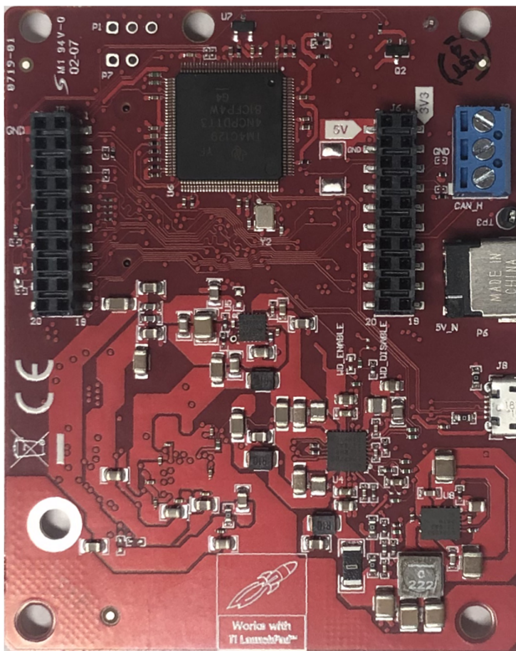
Figure 2. EVM (Rear)
