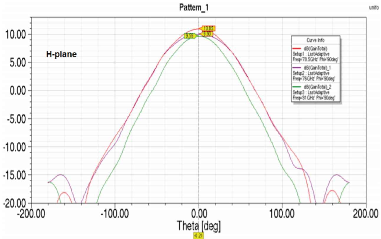
Figure 11. Antenna Pattern
