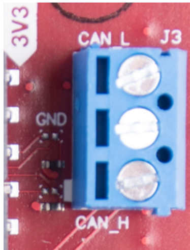
Figure 7. CAN Connector
