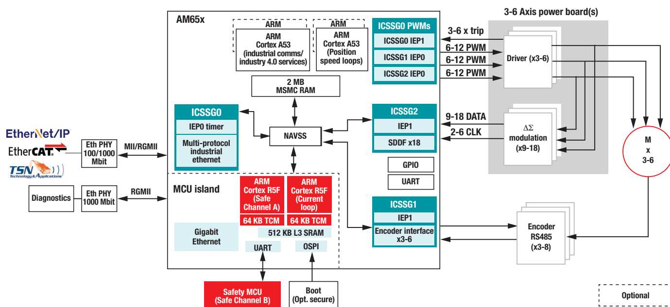
Figure 2. AM65x – Centralized smart servo drive.
