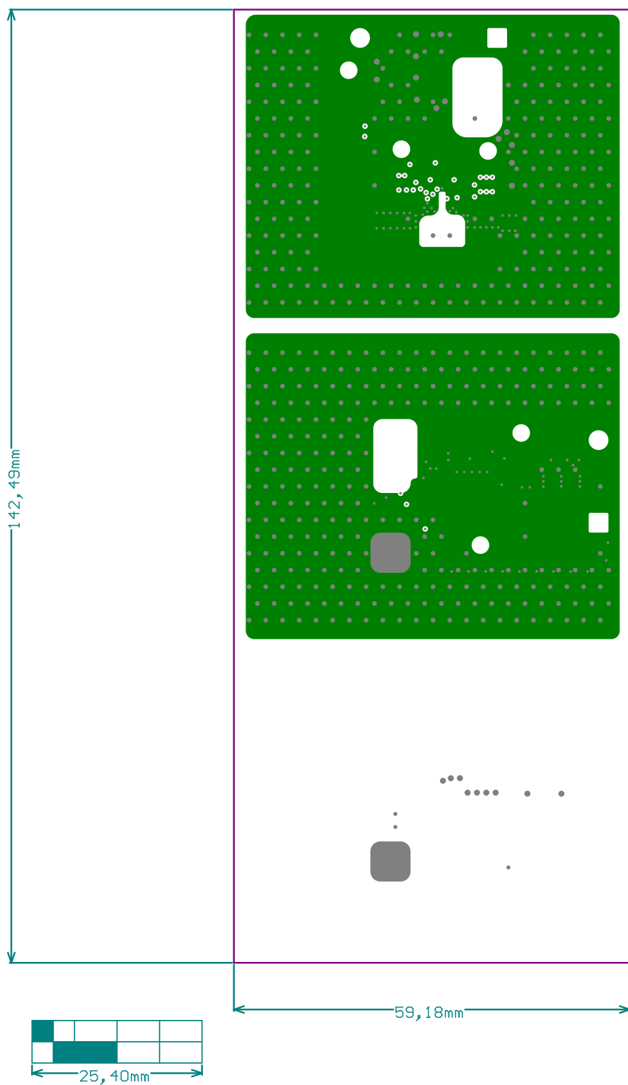
M2 Board Dimensions
