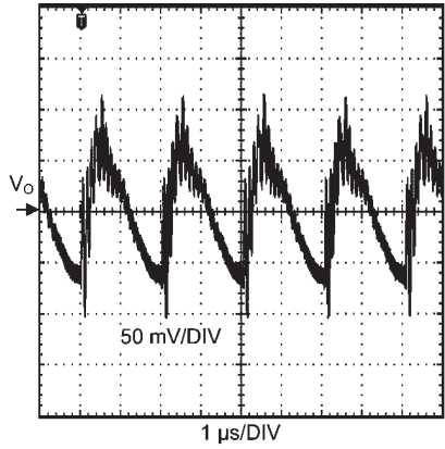
输出电压纹波交流耦合 ( V_{IN} = 9V, I_o = 0.5A )
