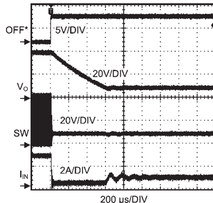
关机 ( V_{IN} = 9V, I_o = 0.5A )
