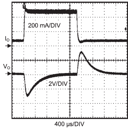
负载瞬态响应 ( V_{IN} = 9V, I_o = 50mA 到 0.5A )
