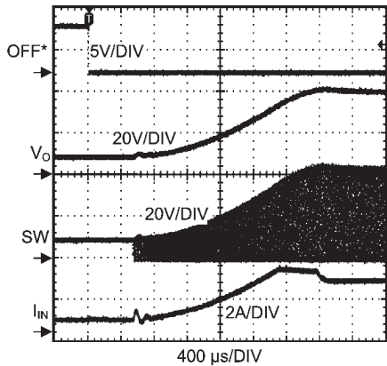
开启 ( V_{IN} = 9V, I_o = 0.5A )
