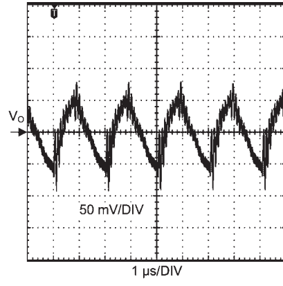
输出电压纹波交流耦合 ( V_{IN} = 16V, I_o = 0.5A )
