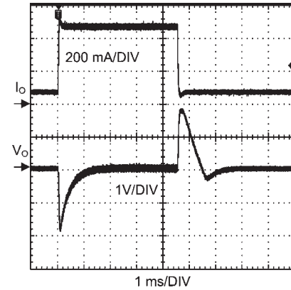
负载瞬态响应 ( V_{IN} = 16V, I_o = 50mA 到 0.5A )
