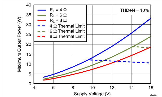
Thermal Limits are referenced to TAS5760xxEVM Rev D
