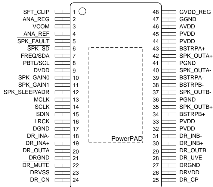
DCA Package 48 Pins TSSOP Top View
