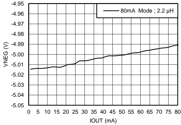
Figure 75. Load Regulation
