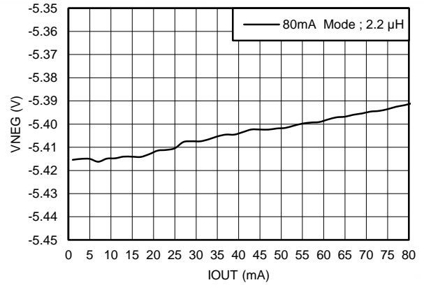
Figure 76. Load Regulation
