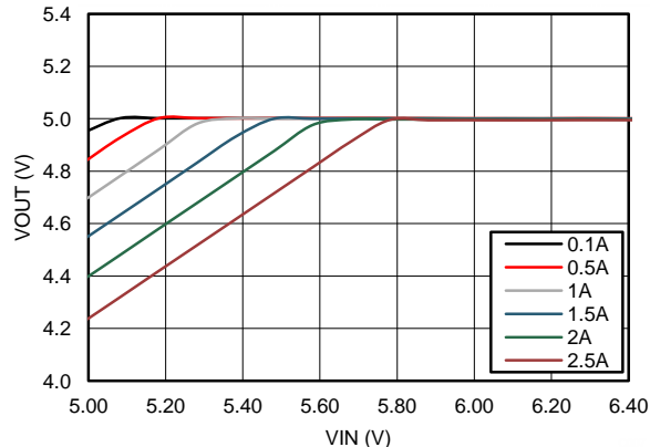
Figure 70. Dropout Curve
