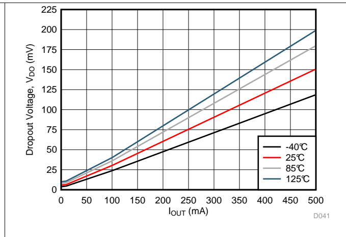
Figure 44. LP5912-1.8 Dropout Voltage ( V_{DO} ) vs I_{OUT}
