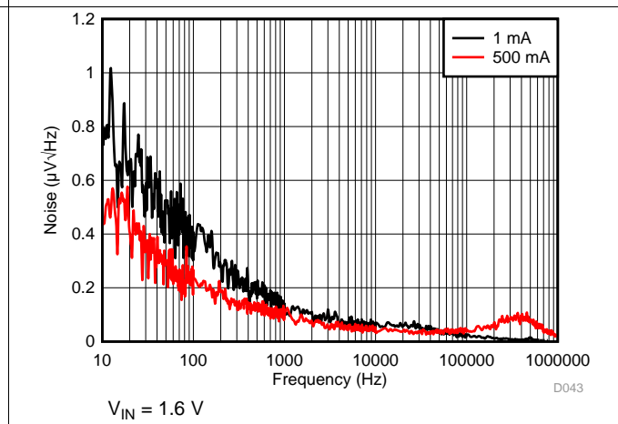
Figure 46. LP5912-0.9 Noise vs Frequency
