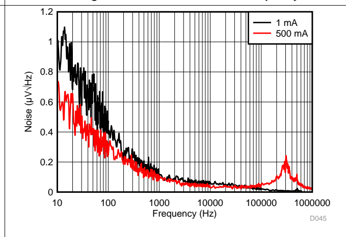
Figure 48. LP5912-3.3 Noise vs Frequency
