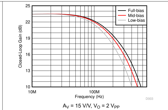
图 5-14. Small-Signal Frequency Response vs Bias Modes
