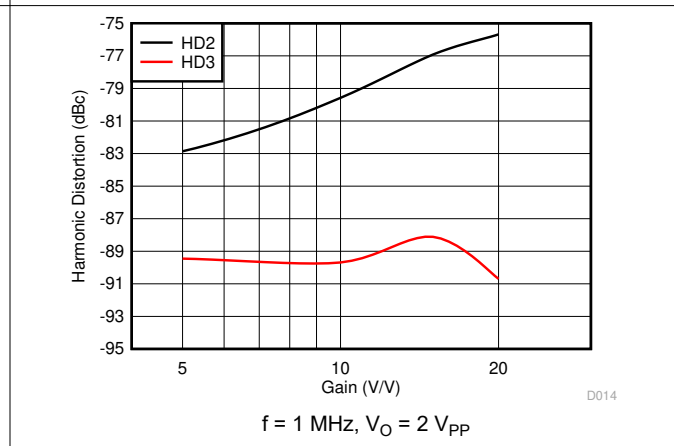
图 5-18. Harmonic Distortion vs Gain
