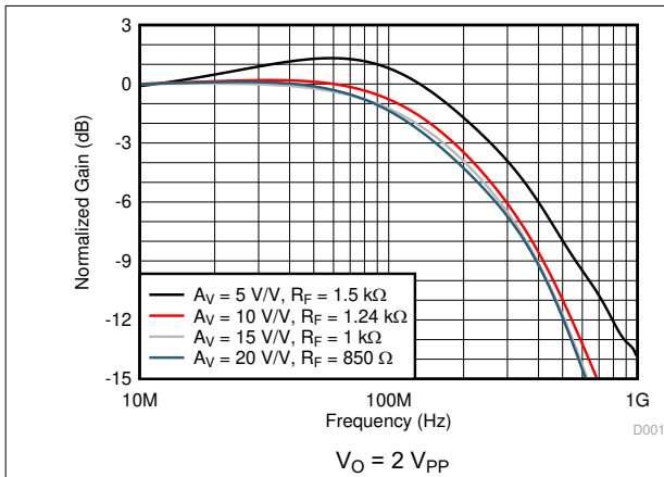
图 5-1. Small-Signal Frequency Response
