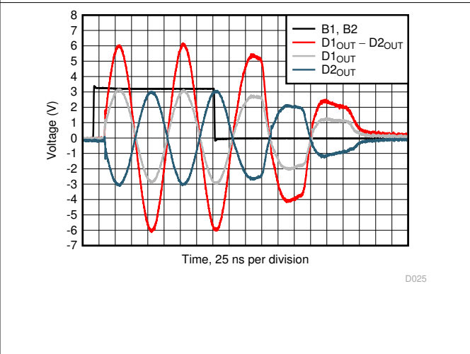
图 5-36. Full-Bias and Shutdown Mode Transition Timing
