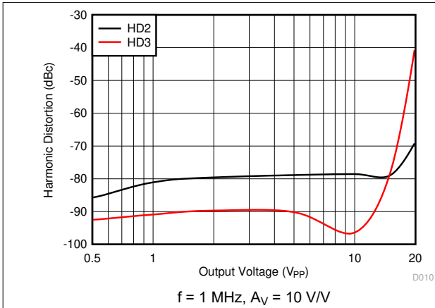
图 5-19. Harmonic Distortion vs V_O
