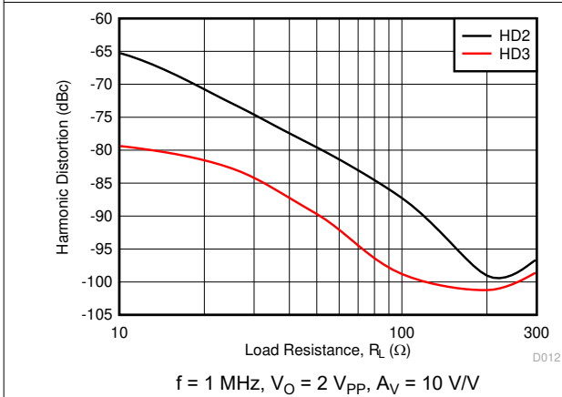
图 5-21. Harmonic Distortion vs R_L
