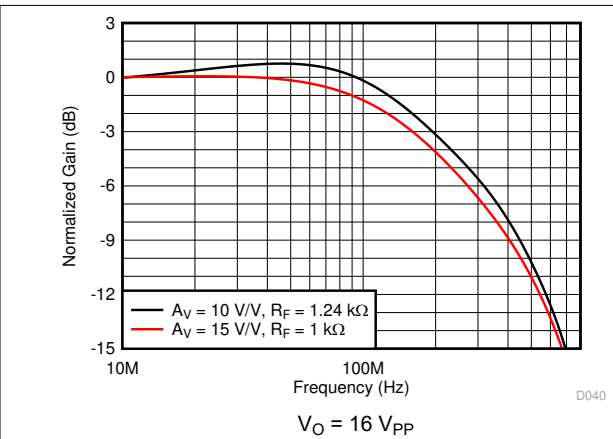
图 5-2. Large-Signal Frequency Response
