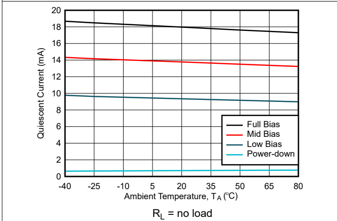
图 5-33. Quiescent Current vs Temperature
