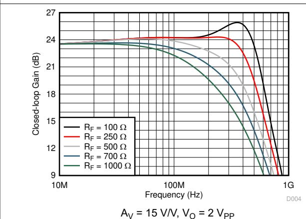
图 5-6. Small-Signal Frequency Response vs R_F
