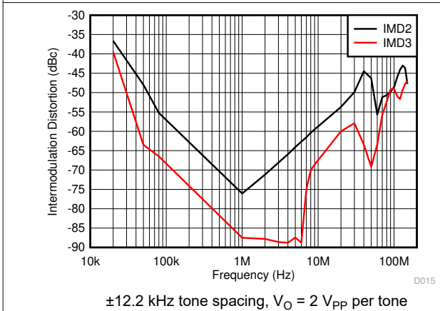
图 5-23. Intermodulation Distortion vs Frequency
