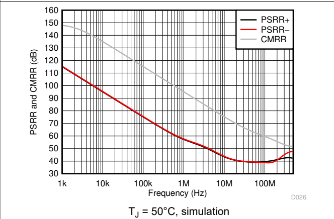
图 5-34. PSRR and CMRR vs Frequency
