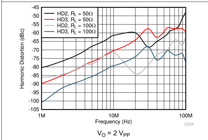
图 5-17. Harmonic Distortion vs Frequency
