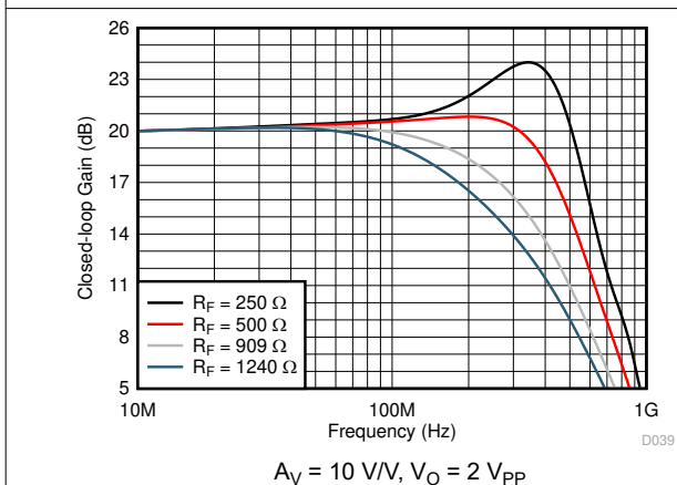
图 5-5. Small-Signal Frequency Response vs R_F
