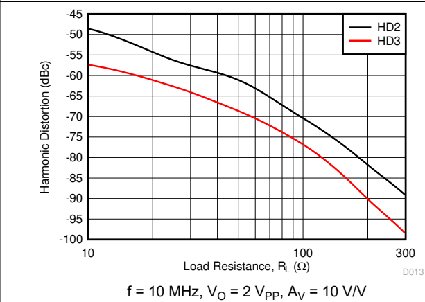
图 5-22. Harmonic Distortion vs R_L
