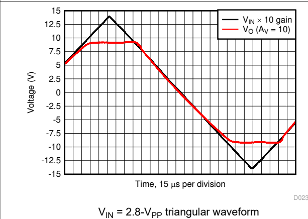
图 5-24. Overdrive Recovery
