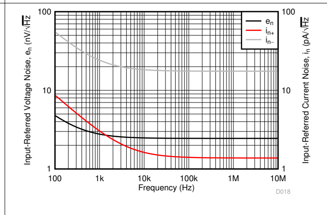
图 5-16. Input Voltage and Current Noise Density vs Frequency
