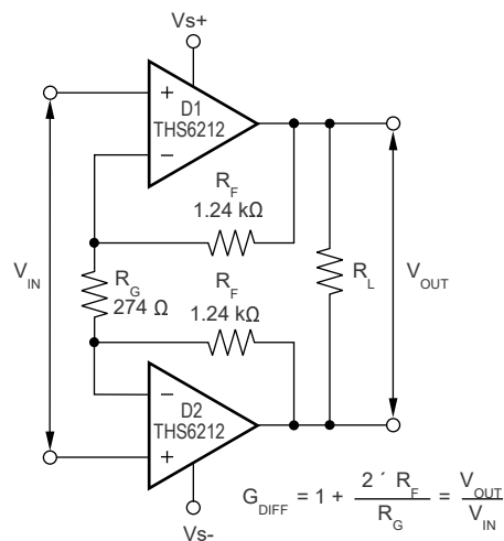
图 7-1. Noninverting Differential I/O Amplifier
