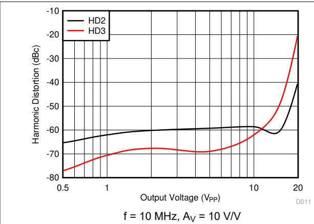
图 5-20. Harmonic Distortion vs V_O
