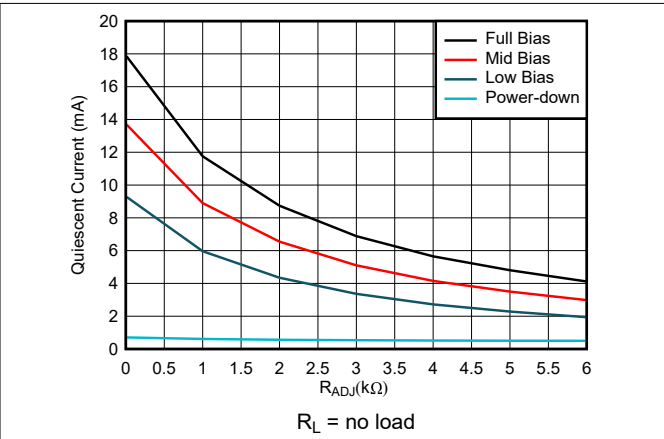
图 5-32. Quiescent Current vs R_{ADJ}
