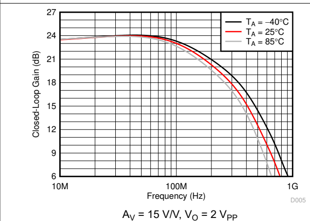
图 5-4. Small-Signal Frequency Response vs Temperature
