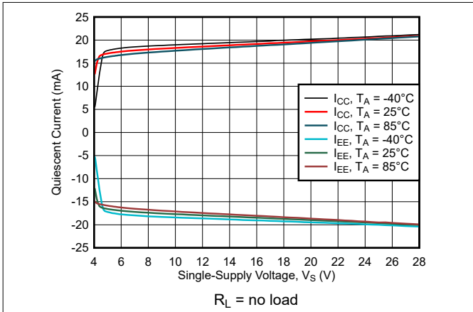
图 5-31. Quiescent Current vs Single-Supply Voltage
