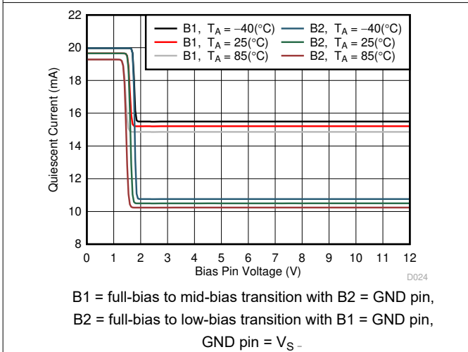
图 5-35. Mode Transition Voltage Threshold
