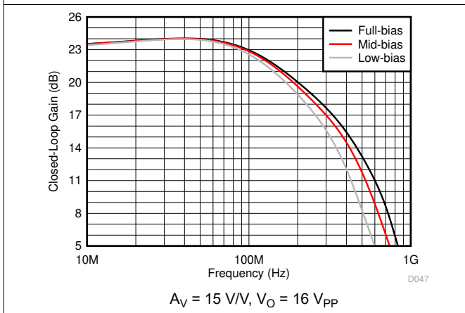
图 5-15. Large-Signal Frequency Response vs Bias Modes
