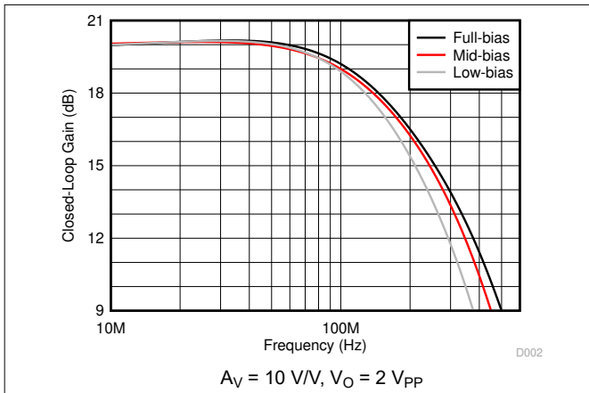
图 5-13. Small-Signal Frequency Response vs Bias Modes
