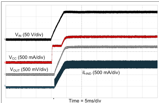
图 28. EN/UVLO Start-up at V_{IN} = 48\text{ V} and I_{OUT} = 1\text{ A}
