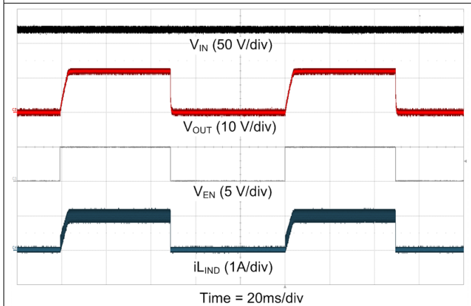
图 30. EN/UVLO Start-up at V_{IN} = 48\text{ V} and R_{LOAD} = 12\ \Omega at FPWM = 1
