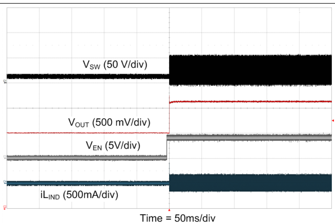
图 29. Pre-Bias (11.5 V) Start-up at V_{IN} = 48\text{ V} at No Load & FPWM = 1
