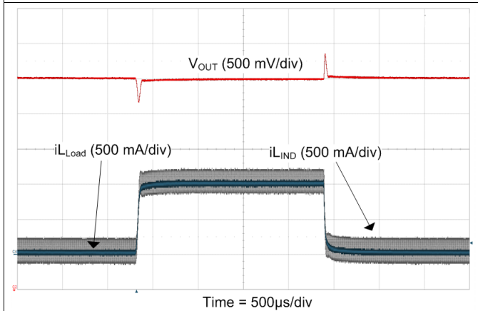
图 32. Load Transient (0 A - 1 A) at V_{IN} = 48\text{ V} at FPWM = 1
