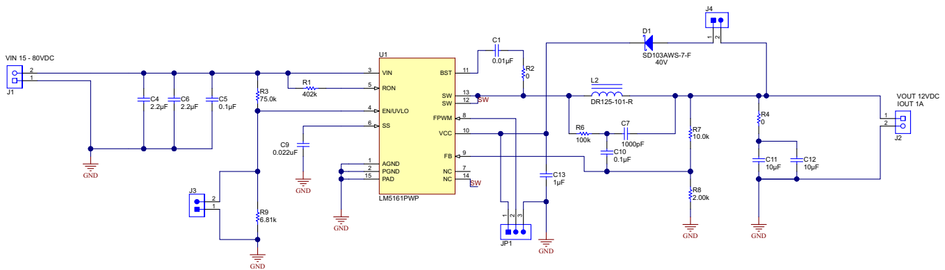
图 25. Synchronous Buck Application Circuit with LM5161
