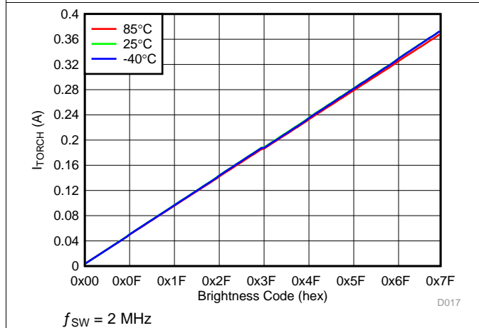
图 18. LED Torch Current vs Brightness Code
