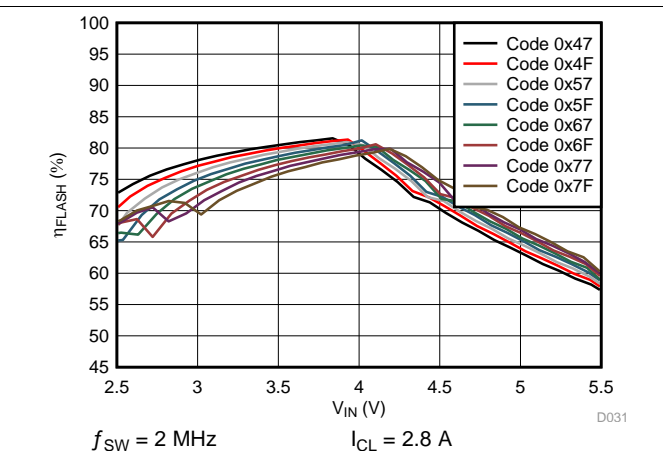
图 41. LED Flash Efficiency vs Input Voltage
