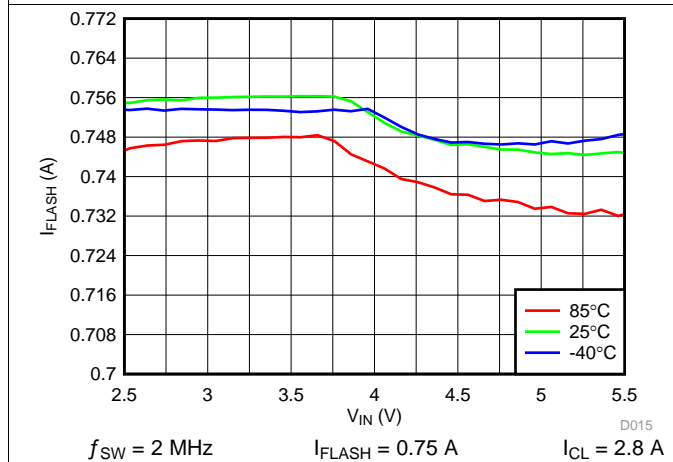
图 16. LED Flash Current vs Input Voltage
