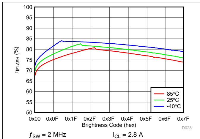
图 38. LED Flash Efficiency vs Brightness Code
