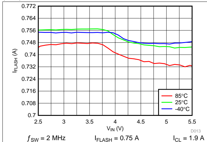
图 14. LED Flash Current vs Input Voltage
