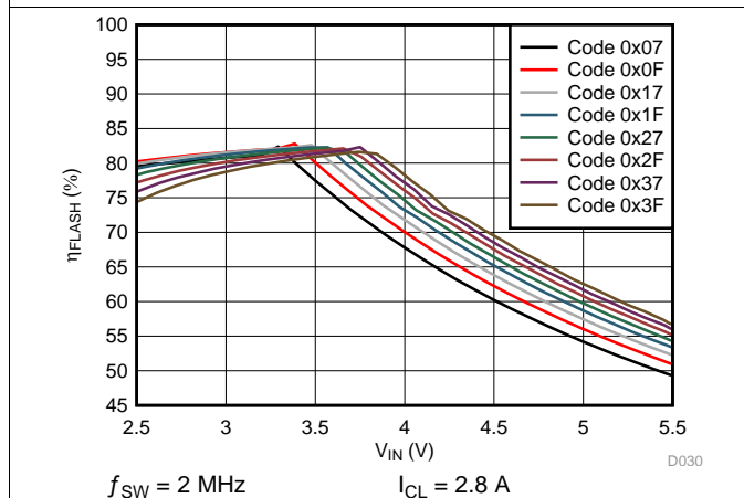
图 40. LED Flash Efficiency vs Input Voltage
