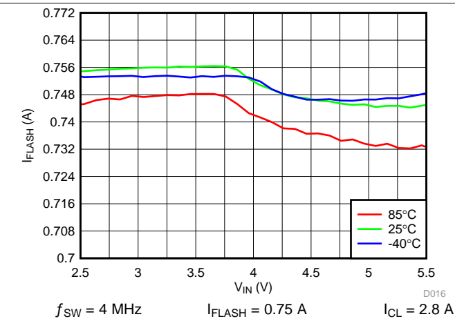
图 17. LED Flash Current vs Input Voltage
