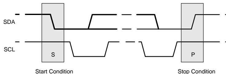
图 34. Start and Stop Conditions
