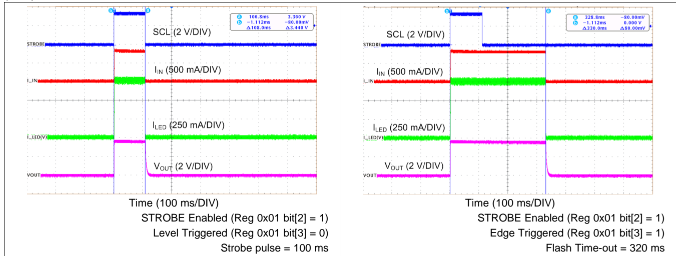
图 68. Flash Turnoff with Level Triggered STROBE
