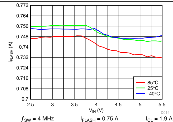
图 15. LED Flash Current vs Input Voltage
