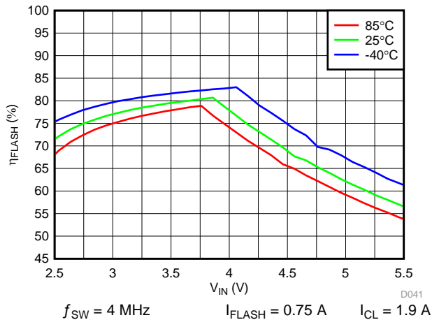
图 51. LED Flash Efficiency vs Input Voltage
