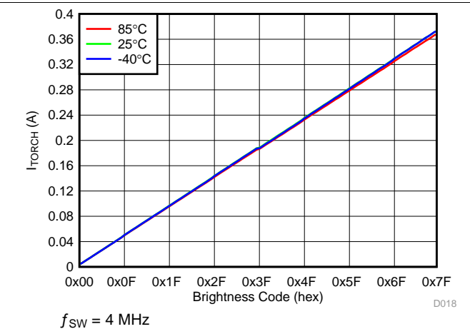
图 19. LED Torch Current vs Brightness Code
