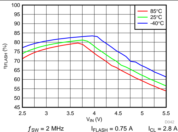
图 52. LED Flash Efficiency vs Input Voltage
