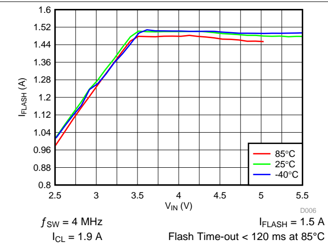
图 7. LED Flash Current vs Input Voltage
