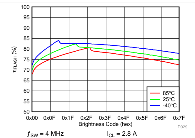
图 39. LED Flash Efficiency vs Brightness Code
