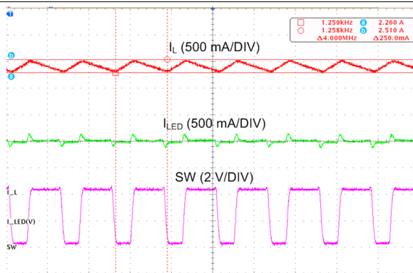
Time (200 ns/DIV) f_{SW} = 4\text{ MHz}
