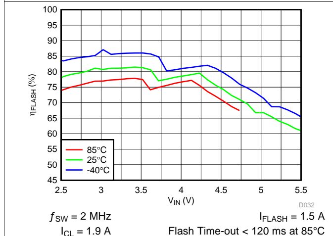
图 42. LED Flash Efficiency vs Input Voltage
