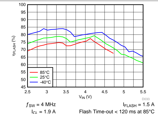
图 43. LED Flash Efficiency vs Input Voltage
