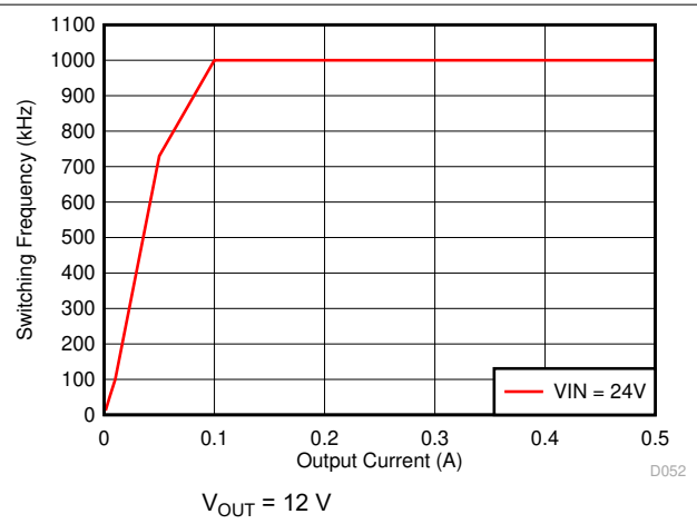
图 7-28. Auto PFM Mode Switching Frequency vs Output Current
