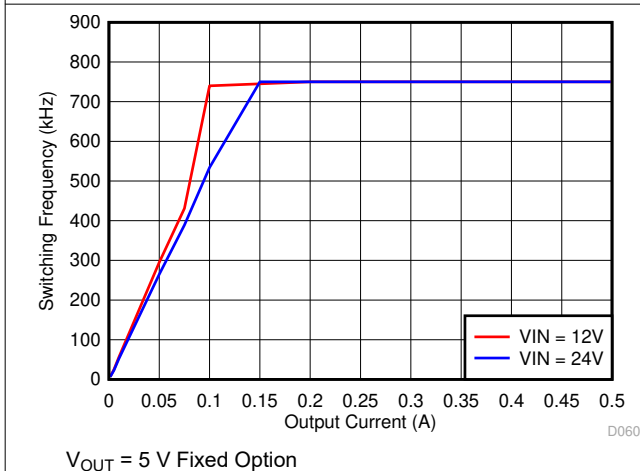
图 7-27. Auto PFM Mode Switching Frequency vs Output Current
