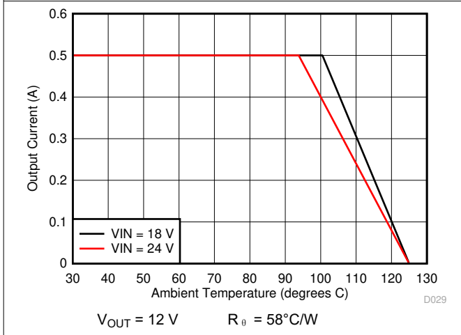
图 7-21. Ambient Temperature vs Output Current
