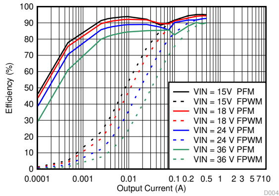
图 9-18. Efficiency
