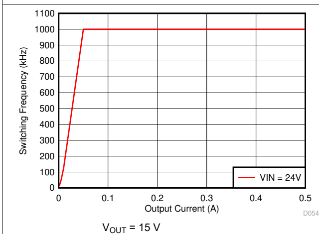
图 7-29. Auto PFM Mode Switching Frequency vs Output Current
