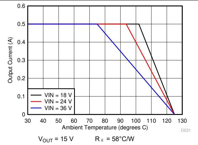
图 7-22. Ambient Temperature vs Output Current
