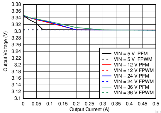
图 9-45. Line and Load Regulation for V_{OUT} = 3.3\text{ V}
