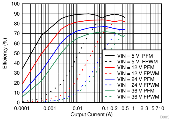
图 9-30. Efficiency
