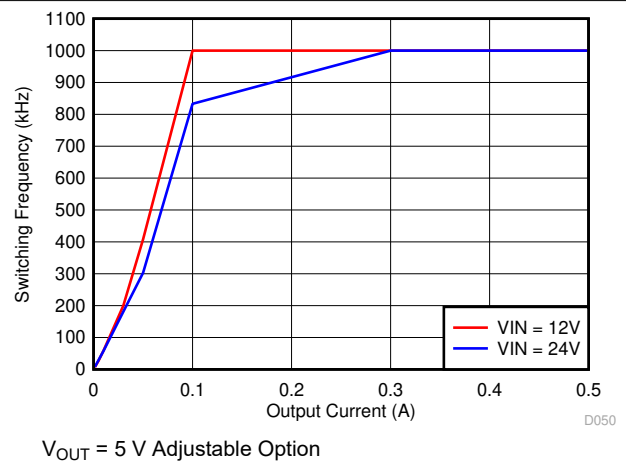
图 7-26. Auto PFM Mode Switching Frequency vs Output Current
