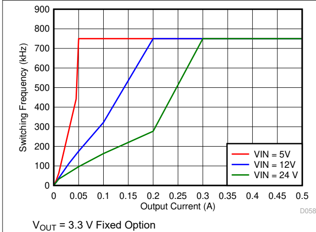
图 7-25. Auto PFM Mode Switching Frequency vs Output Current
