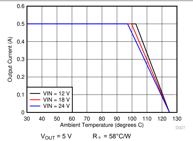
图 7-20. Ambient Temperature vs Output Current
