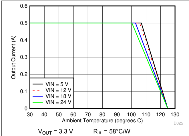
图 7-19. Ambient Temperature vs Output Current
