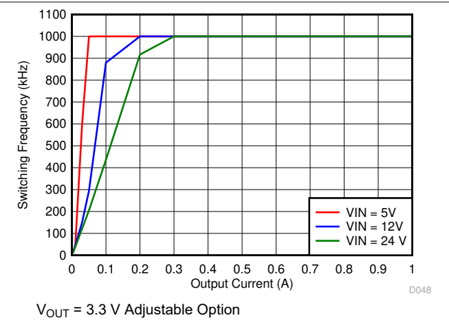
图 7-24. Auto PFM Mode Switching Frequency vs Output Current
