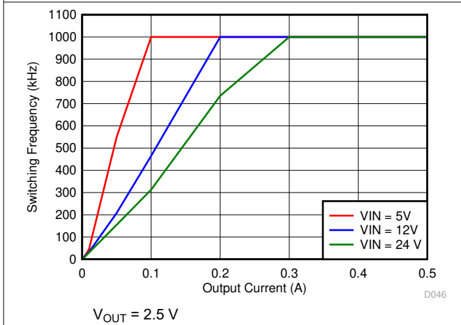
图 7-23. Auto PFM Mode Switching Frequency vs Output Current
