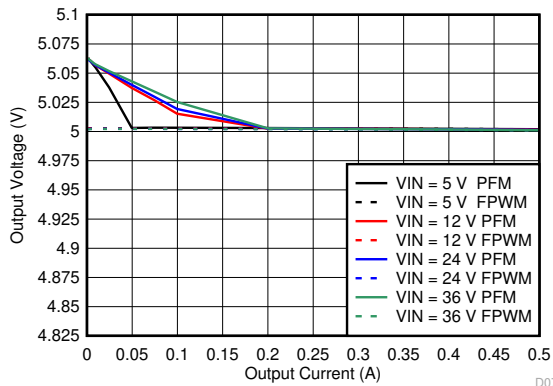
图 9-44. Line and Load Regulation for V_{OUT} = 5\text{ V}
