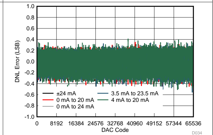
图 37. IOUT DNL vs Code (DC/DC Disabled)
