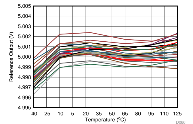
图 71. Internal Reference Voltage vs Temperature
