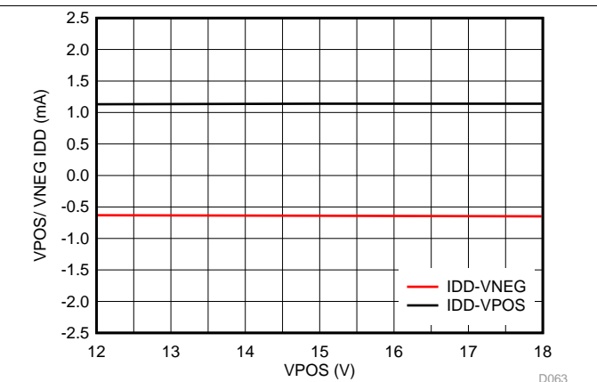
图 69. IOUT Quiescent Current vs VPOS
