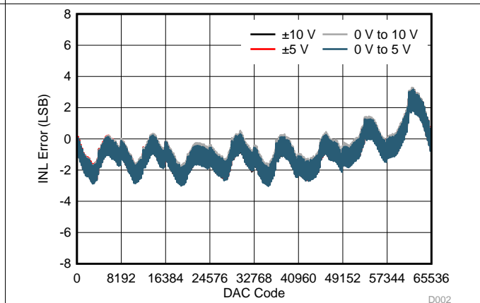
图 6. VOUT INL vs Code (DC/DC Disabled)
