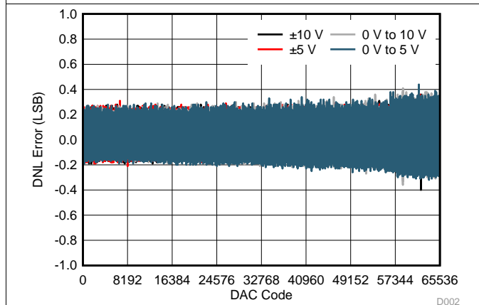
图 5. VOUT DNL vs Code (DC/DC Disabled)
