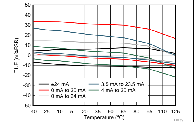
图 43. IOUT TUE vs Temperature
