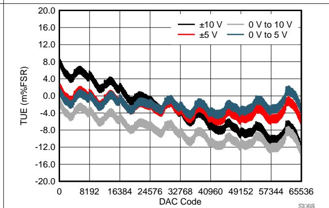
图 8. VOUT TUE vs Code (DC/DC Disabled)
