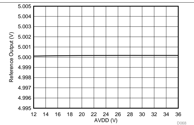
图 73. Internal Reference Voltage vs AVDD
