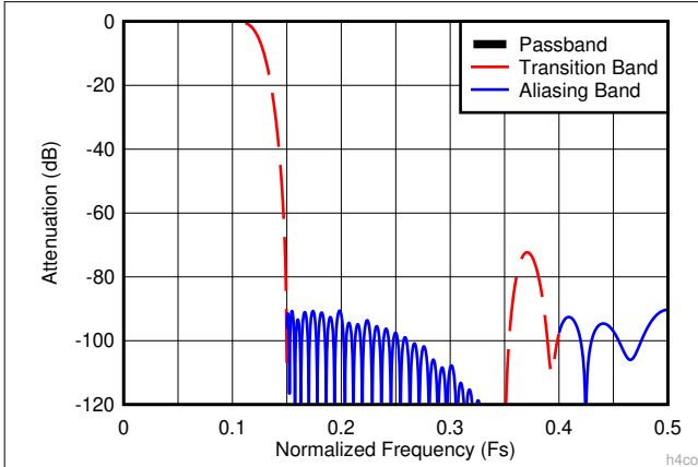
图 7-11. Decimate-by-4 Composite Response
