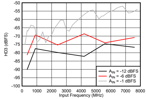
图 6-86. Dual Channel Mode: HD3 vs Input Frequency
