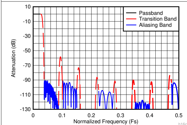
图 7-15. Decimate-by-16 Composite Response
