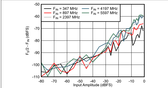
图 6-63. DES Mode: F_S/2 - F_{IN} vs Input Amplitude and Frequency
