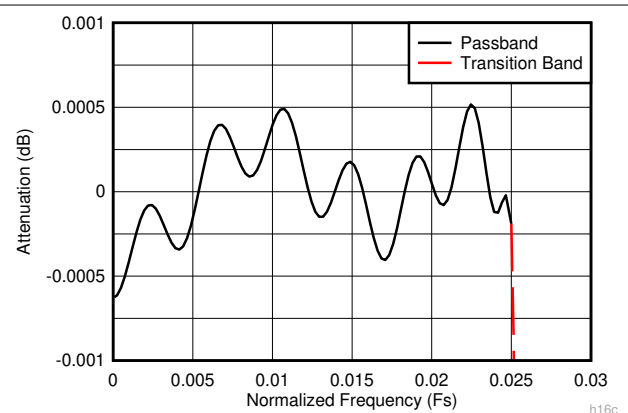
图 7-16. Decimate-by-16 Composite Zoomed Pass-Band Response
