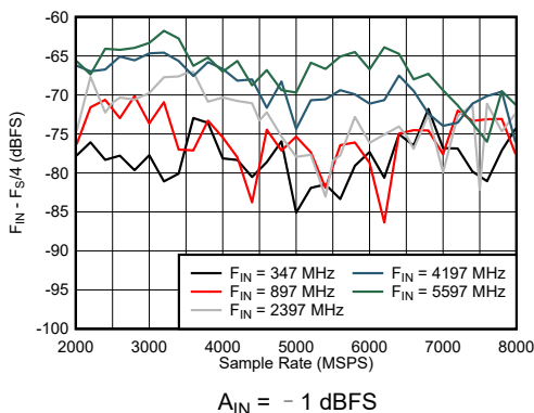
图 6-41. DES Mode: F_{IN} \pm F_S/4 vs Sample Rate and Input Frequency
