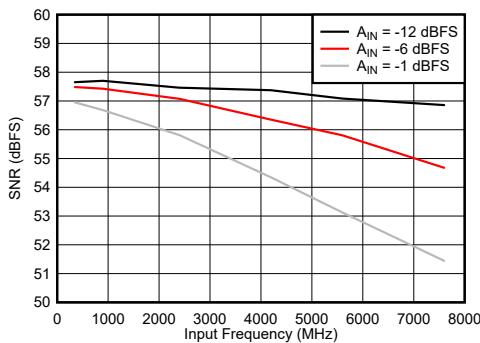
图 6-77. DES Mode: SNR vs Input Frequency
