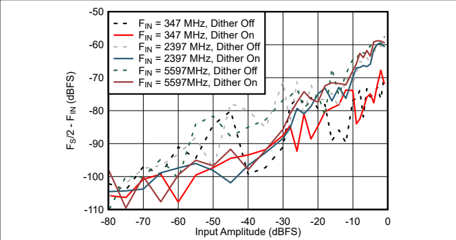
图 6-64. DES Mode: F_S/2 - F_{IN} vs Input Amplitude and Dither
