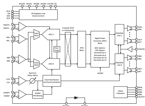
ADC12DJ4000RF 方框图
