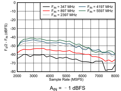
图 6-40. DES Mode: F_S/2 - F_{IN} vs Sample Rate and Input Frequency
