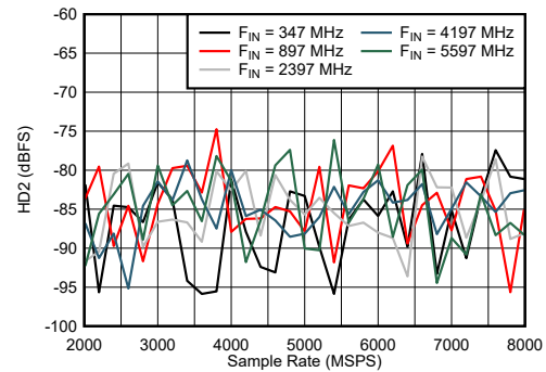
图 6-34. DES Mode: HD2 vs Sample Rate and Input Frequency
