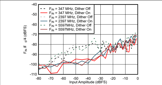
图 6-66. DES Mode: F_{IN} \pm F_{IN}/4 vs Input Amplitude and Dither
