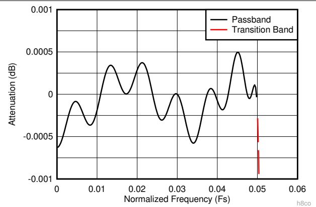
图 7-14. Decimate-by-8 Composite Zoomed Pass-Band Response
