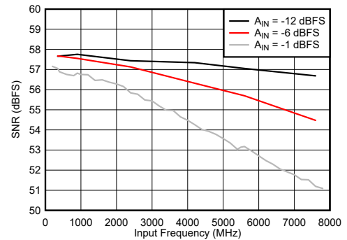
图 6-82. DES Mode: F_{IN} \pm F_S/4 vs Input Frequency
