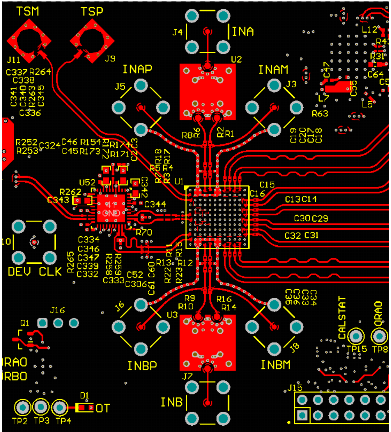
图 8-6. Top Layer Routing: Analog Inputs, CLK and SYSREF, DA0-3, DB0-3
