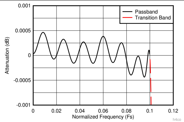
图 7-12. Decimate-by-4 Composite Zoomed Pass-Band Response
