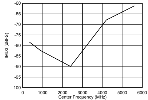
图 6-104. DES Mode: IMD3 vs Input Frequency
