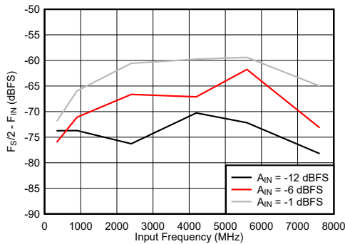
图 6-81. DES Mode: F_S/2 - F_{IN} vs Input Frequency
