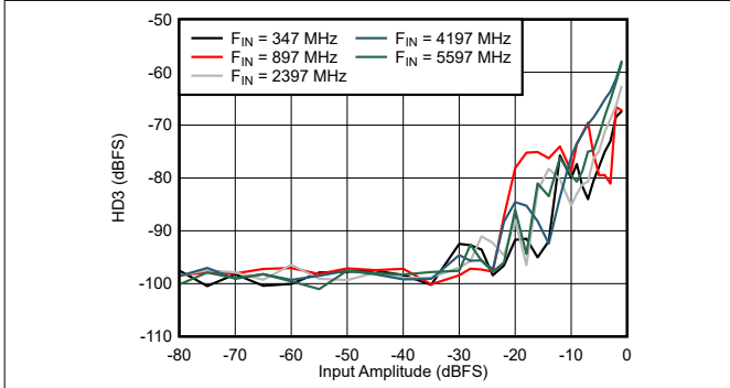
图 6-61. DES Mode: HD3 vs Input Amplitude and Frequency
