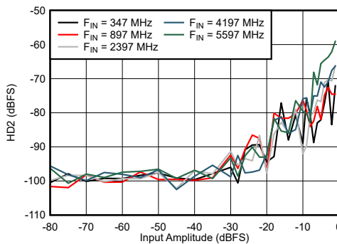
图 6-71. Dual Channel Mode: HD2 vs Input Amplitude and Frequency
