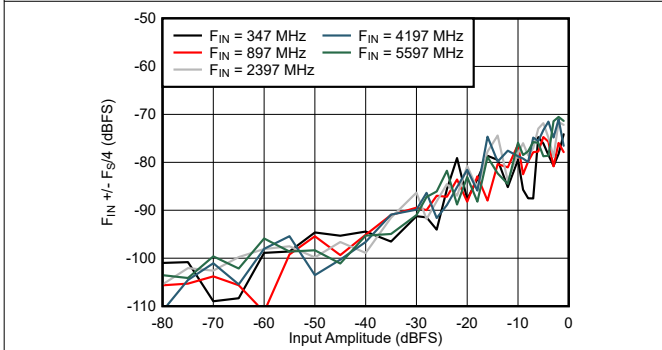
图 6-65. DES Mode: F_{IN} \pm F_{IN}/4 vs Input Amplitude and Frequency
