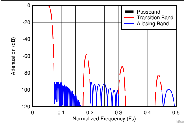
图 7-13. Decimate-by-8 Composite Response
