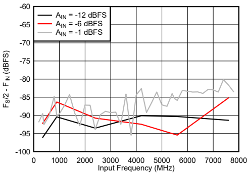
图 6-87. Dual Channel Mode: F_S/2 - F_{IN} vs Input Frequency
