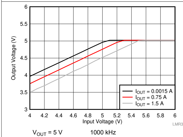
图 10-30. Overall Dropout Characteristic
