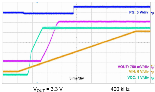
图 10-15. Start-Up Waveform
