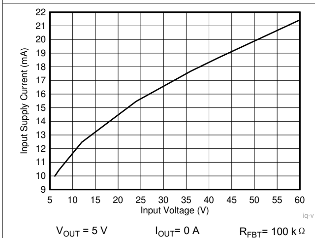
图 10-32. Input Supply Current
