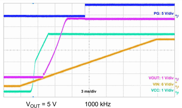
图 10-33. Start-Up Waveform
