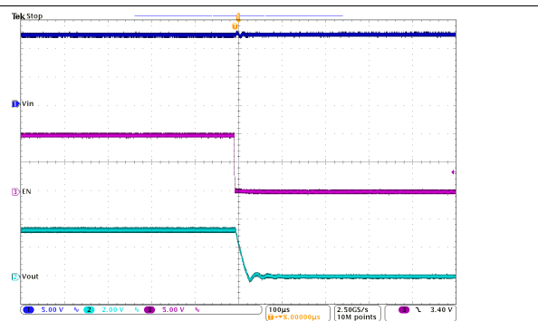
I_{OUT} = 3 A
