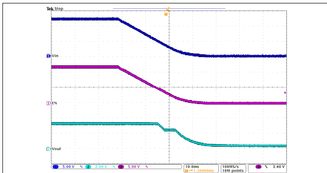
I_{OUT} = 0 A
