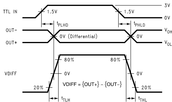
图 10. Differential Driver Propagation Delay and Transition Time Waveforms
