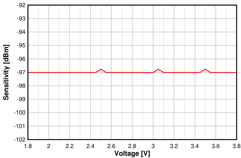
图 8-16. Sensitivity vs. Supply Voltage (VDDS) (BLE 1 Mbps, 2.44 GHz, DCDC Off)
