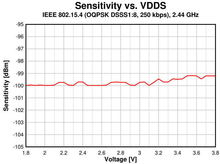
图 8-17. Sensitivity vs. Supply Voltage (VDDS) IEEE 802.15.4 (OQPSK DSSS1:8, 250 kbps)
