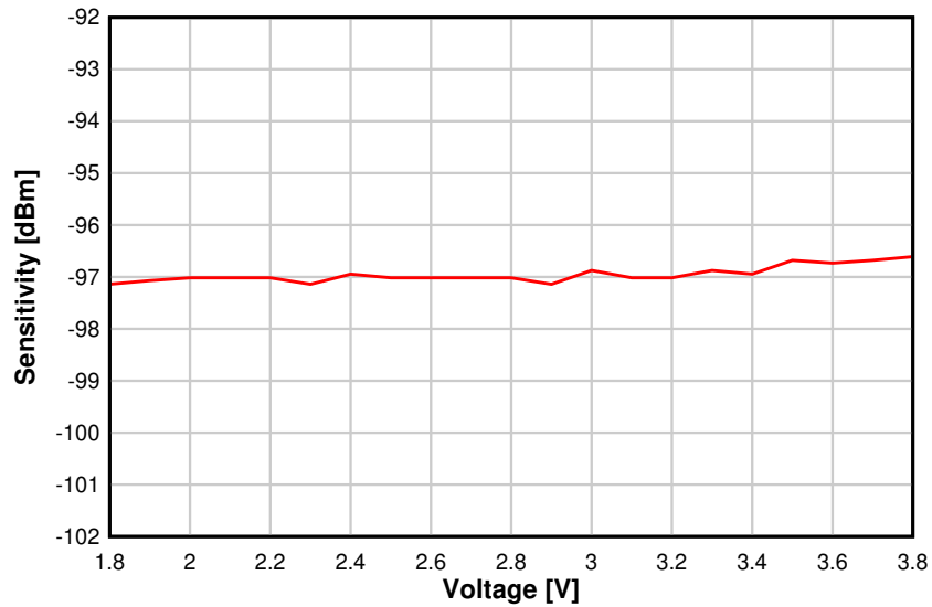
图 8-15. Sensitivity vs. Supply Voltage (VDDS) (BLE 1 Mbps, 2.44 GHz)
