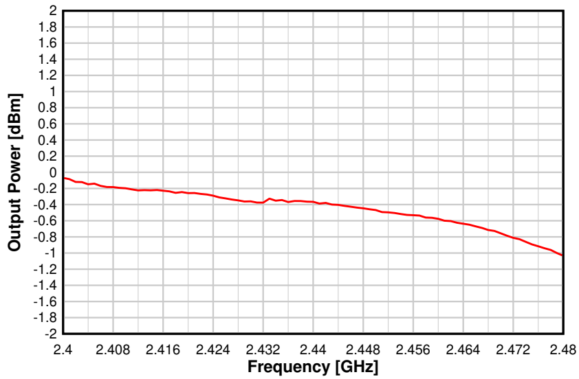
图 8-22. Output Power vs. Frequency (BLE 1 Mbps, 2.44 GHz, 0 dBm)
