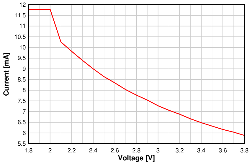
图 8-8. RX Current vs. Supply Voltage (VDD5) (BLE 1 Mbps, 2.44 GHz)
