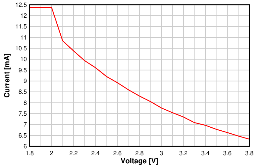
图 8-10. TX Current vs. Supply Voltage (VDD5) (BLE 1 Mbps, 2.44 GHz)
