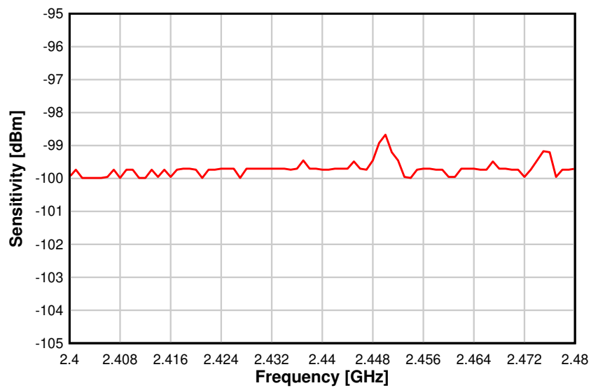
图 8-12. Sensitivity vs. Frequency IEEE 802.15.4 (OQPSK DSSS1:8, 250 kbps)
