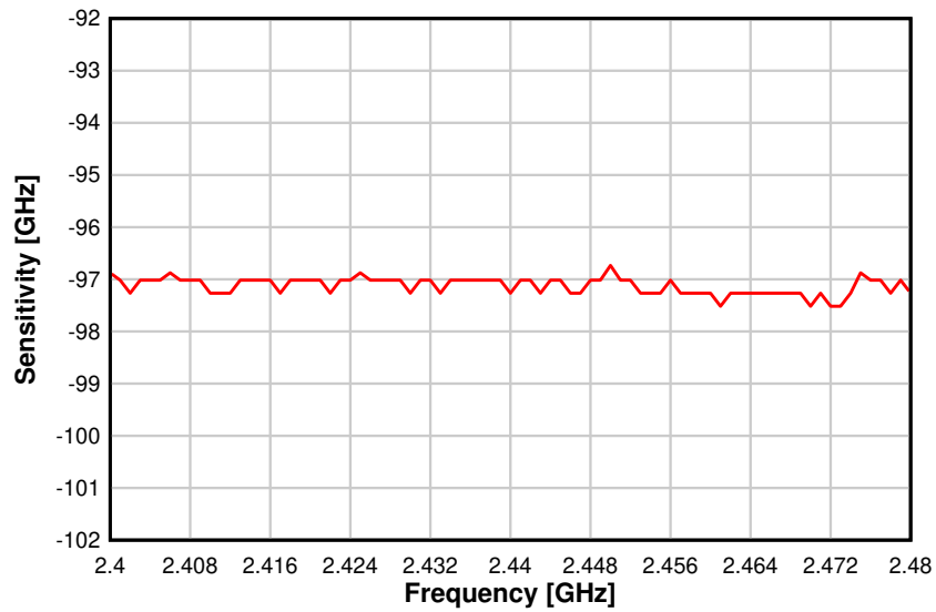
图 8-11. Sensitivity vs. Frequency (BLE 1 Mbps, 2.44 GHz)
