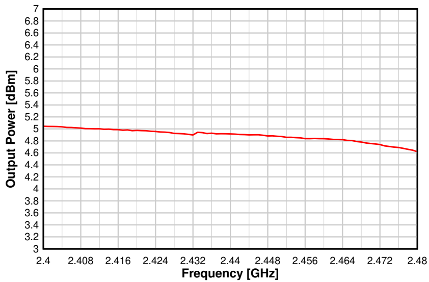
图 8-23. Output Power vs. Frequency (BLE 1 Mbps, 2.44 GHz, +5 dBm)
