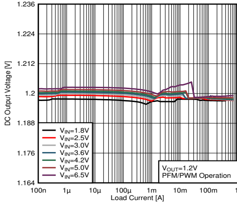
图 26. Output Voltage versus Load Current V OUT = 1.2 V
