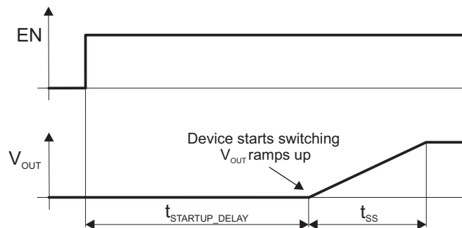
图 12. Device Start-up
