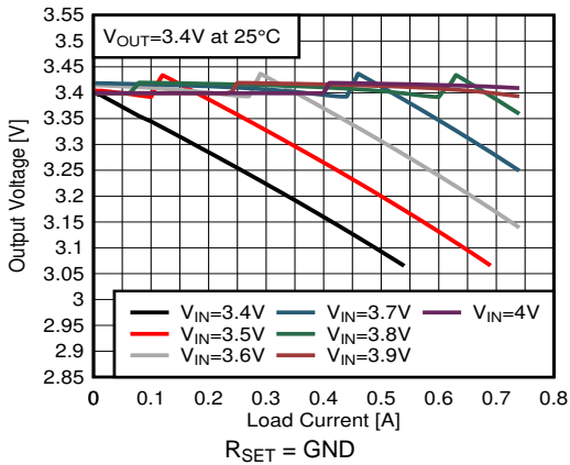
图 30. Output Voltage versus Load Current V OUT = 3.4 V
