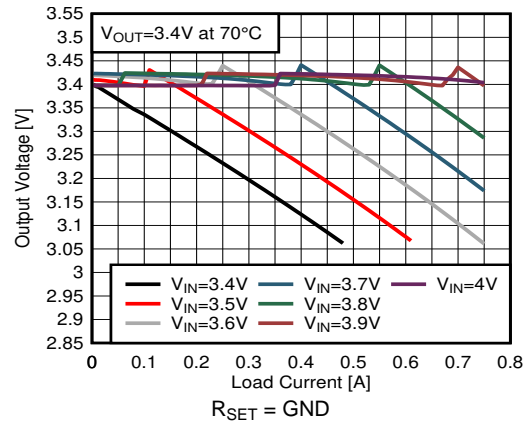
图 31. Output Voltage versus Load Current V OUT = 3.4 V
