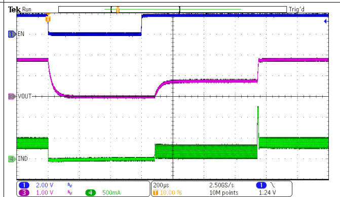
图 53. 100% Mode Entry/Exit Operation
